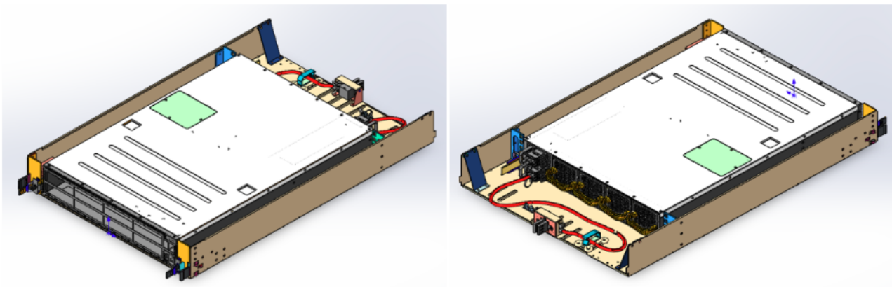
Figure 6: 1RU QFX5140-24CD80 Switch in a 10U ORv3 Tray QFX514024CD8ODO-T1
