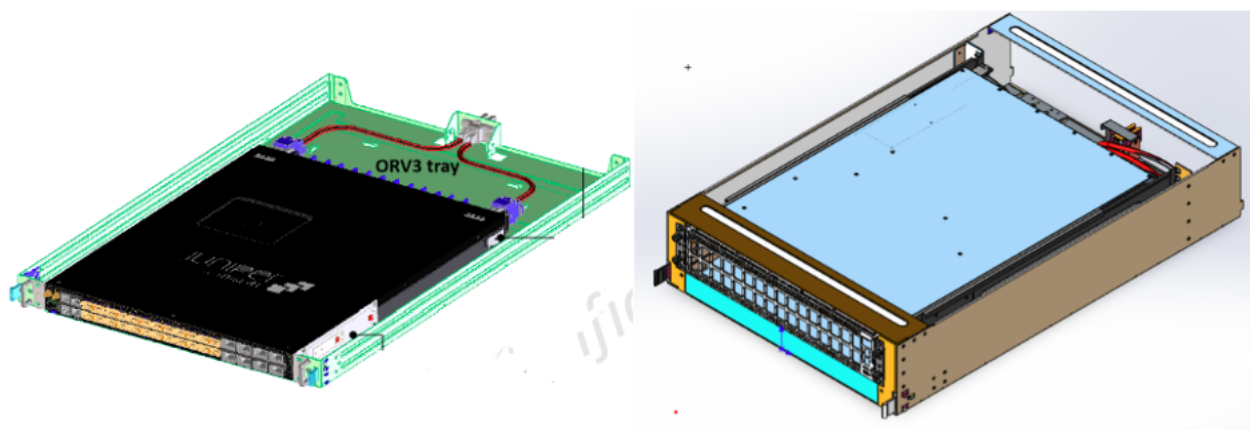
Figure 7: RU Air cooled QFX5250-64OE Switch in a 30U ORv3 Tray QFX5250-64OE-DO-T3
