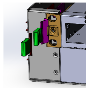
Fig 6: Native ORv3 Platforms Switch to Tray Spring Latch
