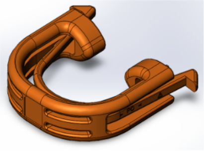
Fig 3: New Fan Handle with Tool Less Locking
