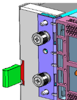
Fig 4: Retrofit Platforms Switch to Tray Thumbscrew
