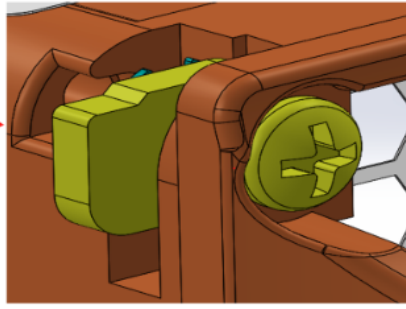
Fig 2: Locking Mechanism of the Existing Fans
