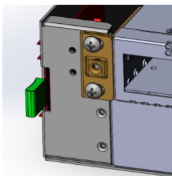
Fig 5: Retrofit Platforms Switch to Tray Loose Screws
