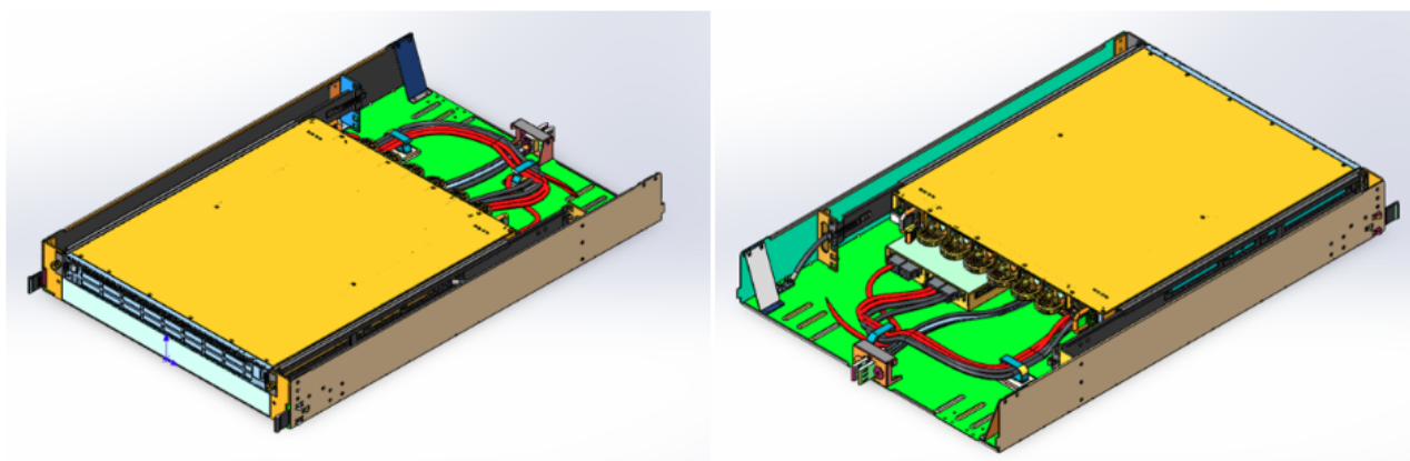
Figure 4: Design Diagrams for QFX513032CDDAFO-T2 and QFX522032CDDAFO-T2
