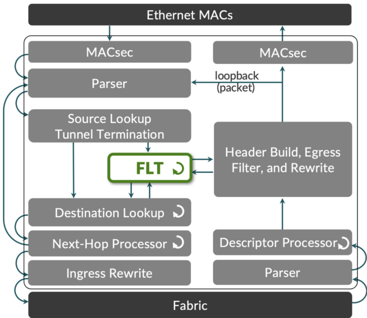
Figure 6: High-Level Description of the Express PFE Architecture
