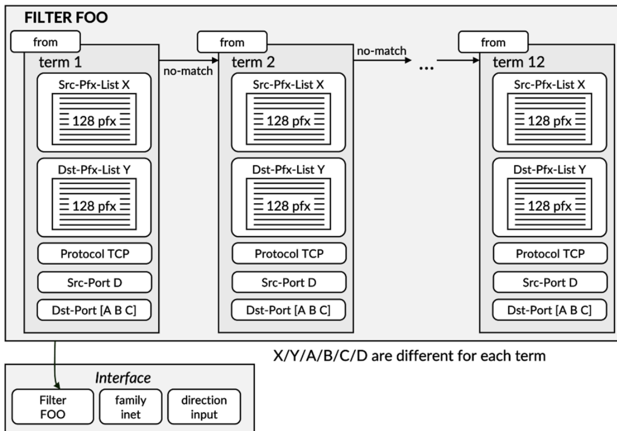
Figure 13: Design of this filter
