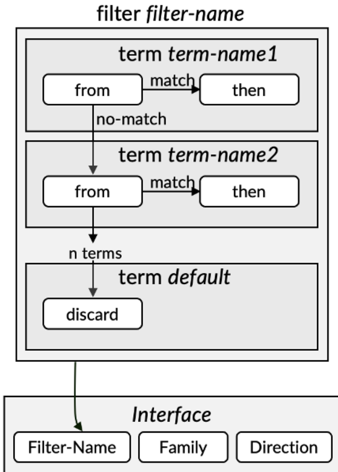
Figure 1: High-Level Description of a Firewall Filter
