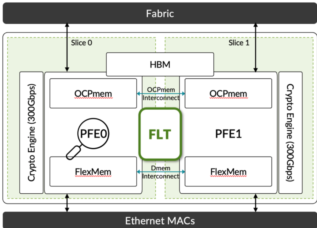
Figure 9: FLT in Trio ASICs
