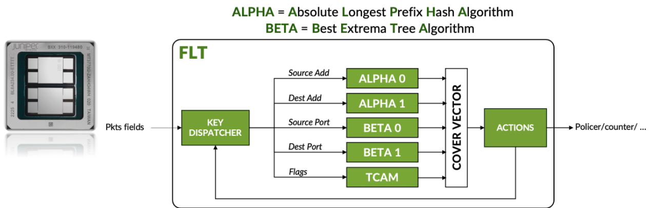
Figure 7: Inside the Express FLT Block
