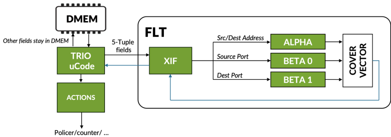
Figure 10: FLT in Trio ASICs
