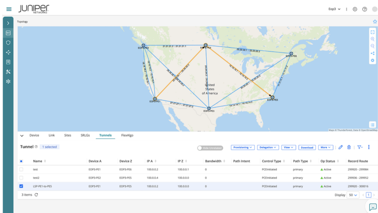
Figure 11: SR LSP tunnel back to normal.
