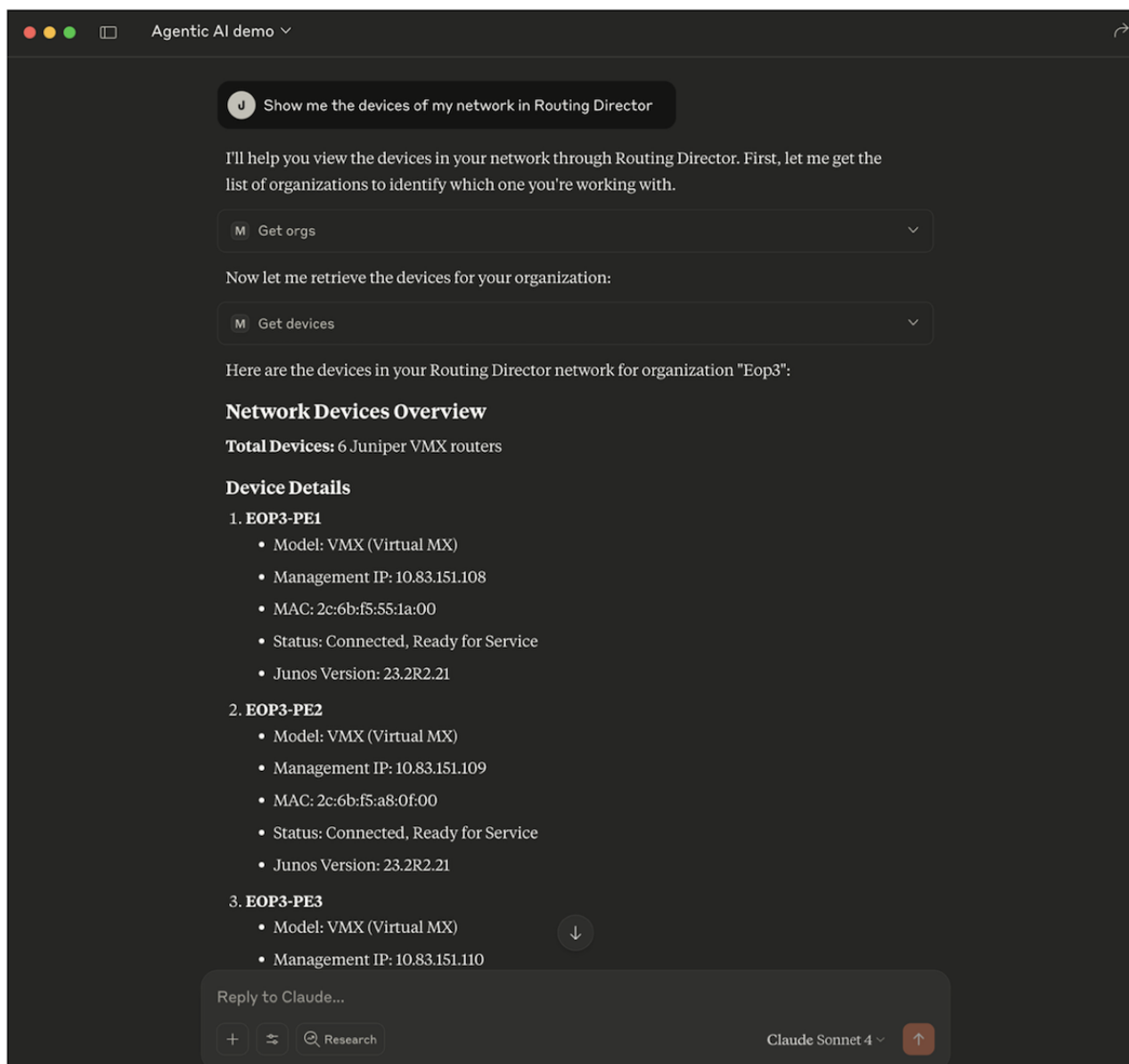
Figure 4: Inventory discovered by AI agent.
