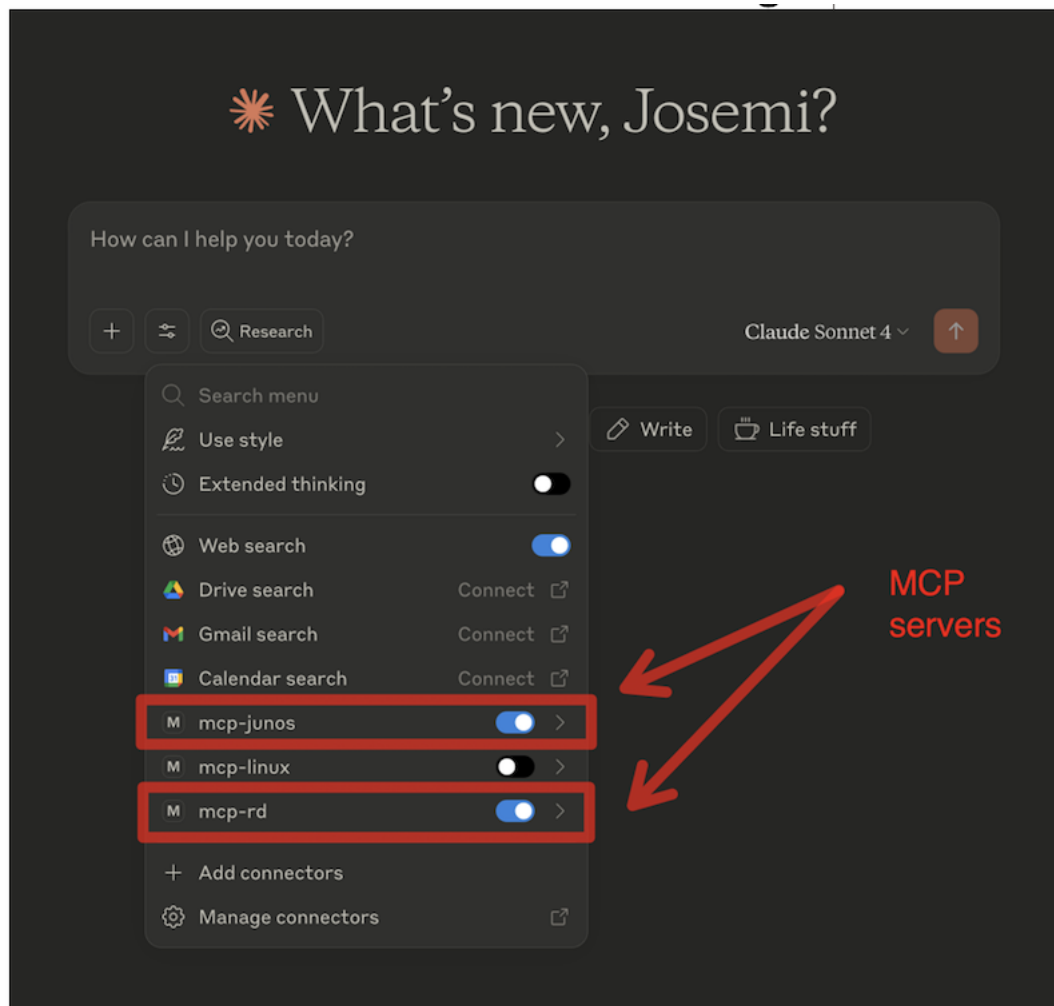
Figure 2: MCP Servers configured in Claude Desktop app.
