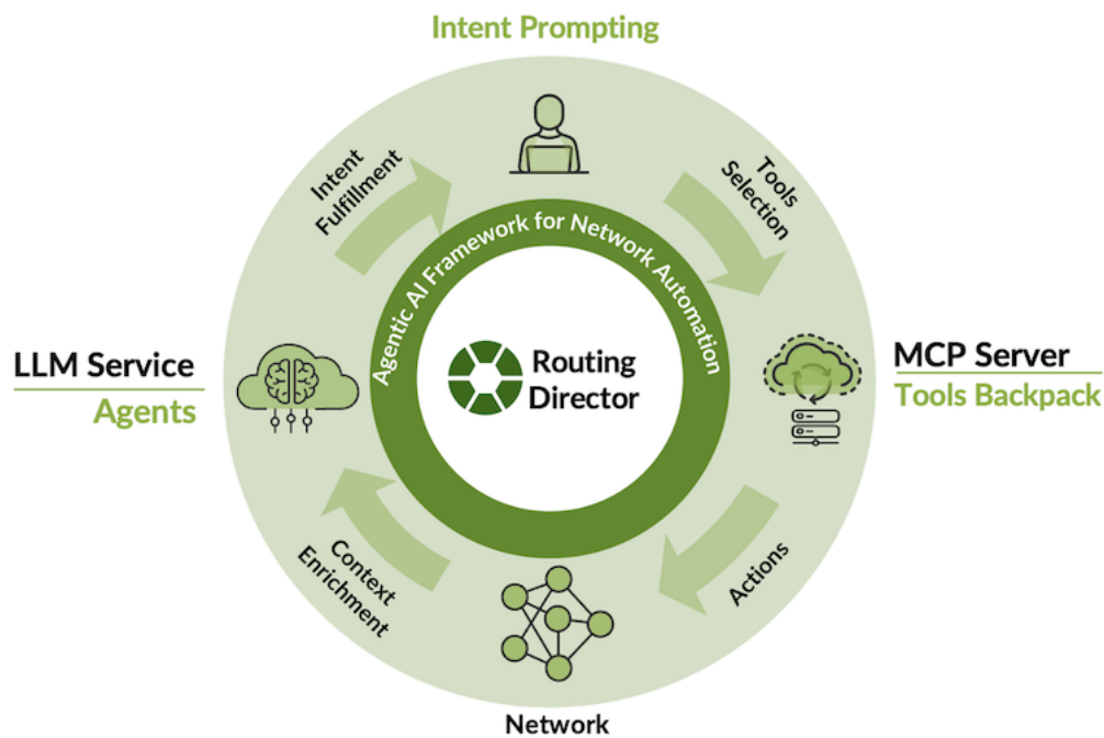
Figure 3: AIOps workflow.
