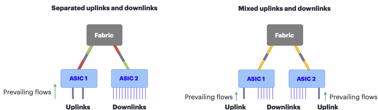
Figure 2: Aggregation router fabric utilization, mixing uplinks vs. separating them.
