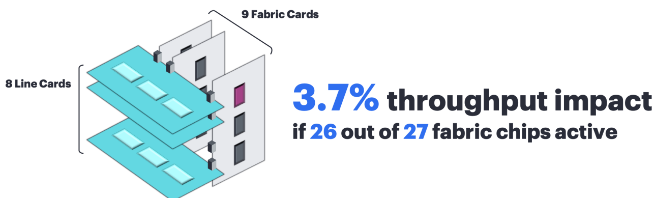
Figure 4: PTX12008 line card and fabric card configuration with one fabric chip less
