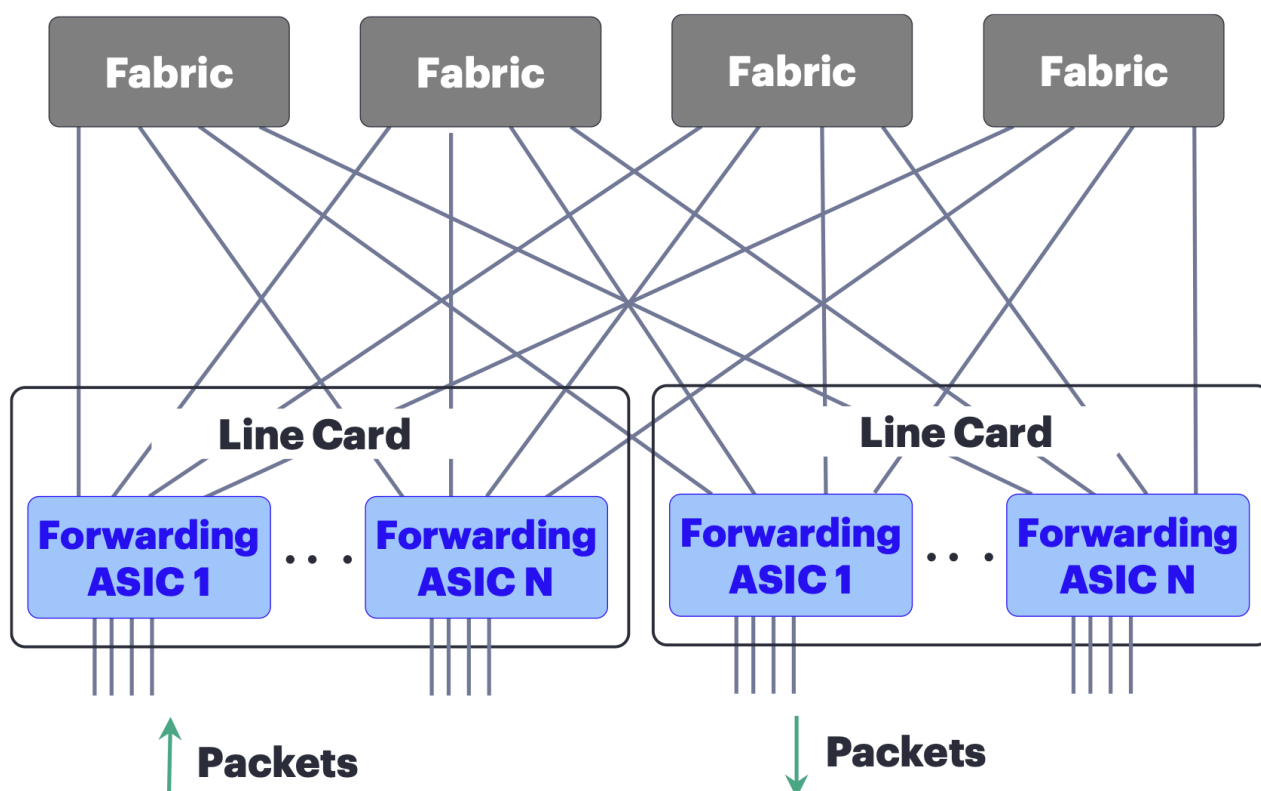
Figure 1: Distributed forwarding system architecture.
