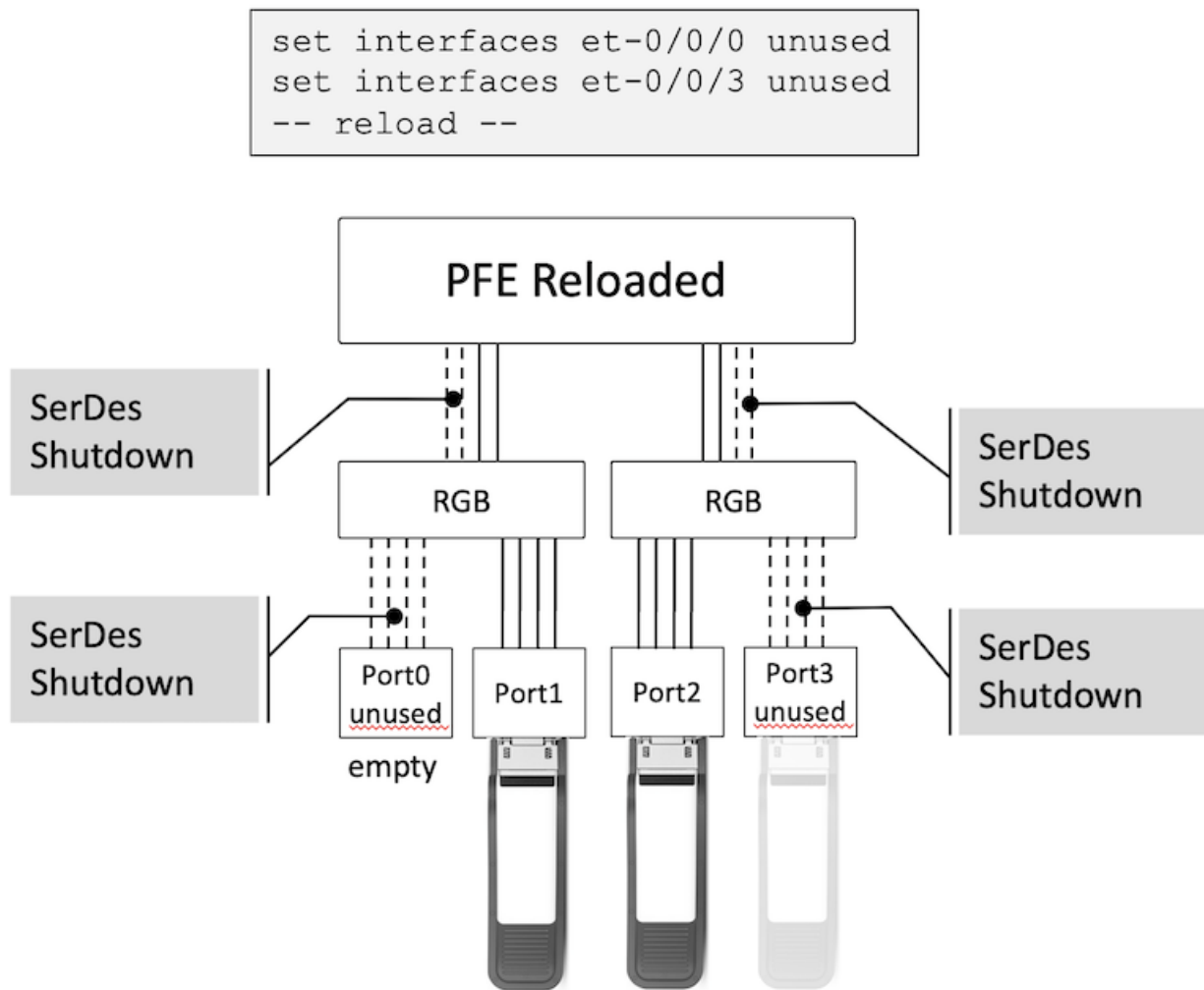
Figure 4: Configuring “Unused” on Ports Connected via a PHY and System Restart
