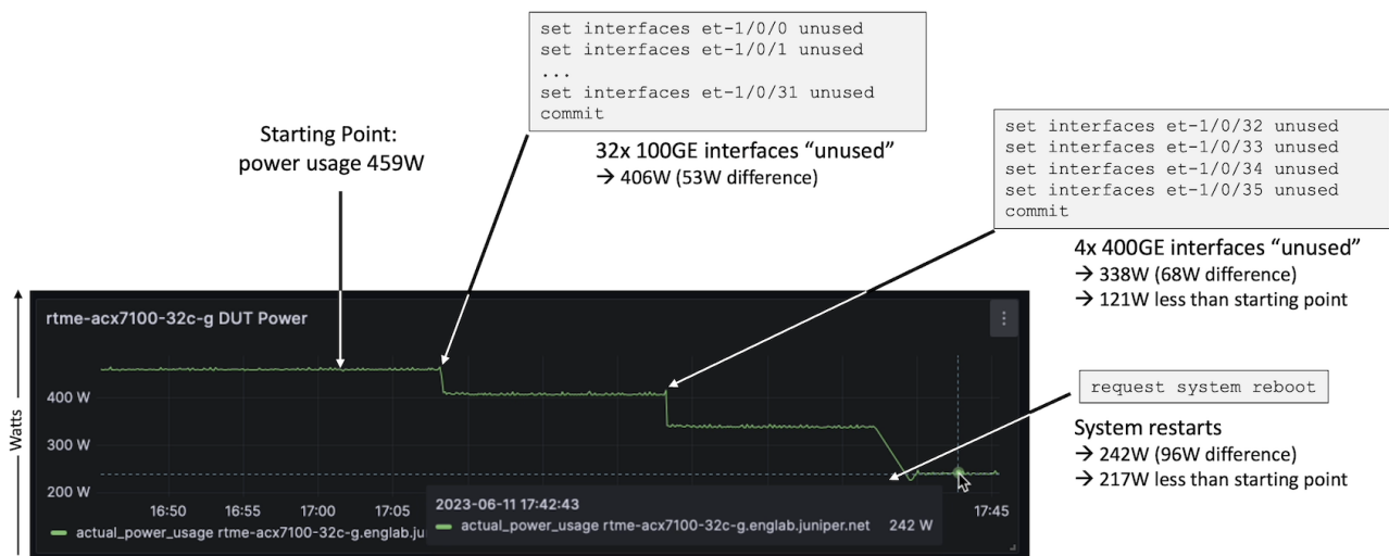
Figure 9: Power Saving Tests on ACX7100-32C
