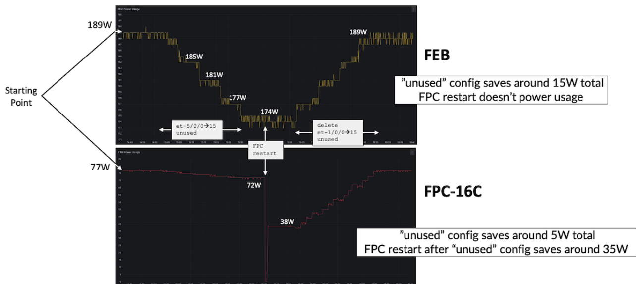
Figure 12: Power Saving Tests on ACX7509 with FPC-16C
