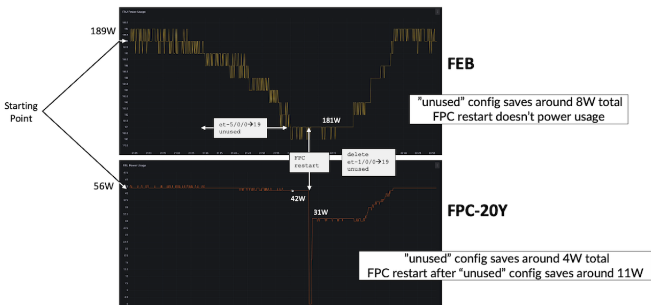
Figure 13: Power Saving Tests on ACX7509 with FPC-20Y
