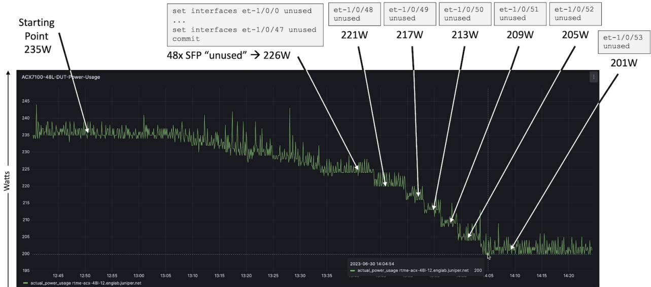
Figure 8: Power Saving Tests on ACX7100-48L
