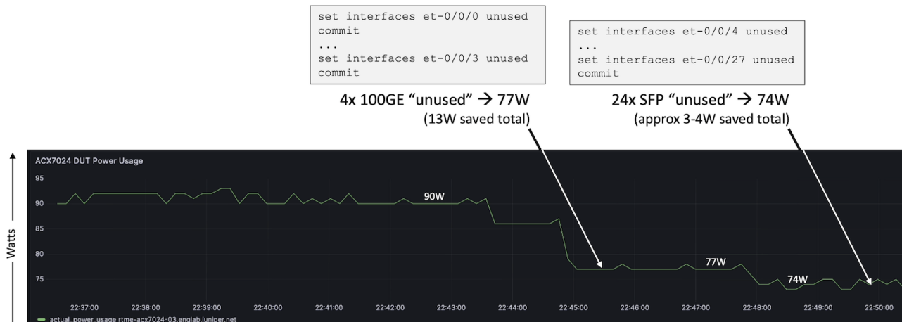
Figure 7: Power Saving Tests on ACX7024
