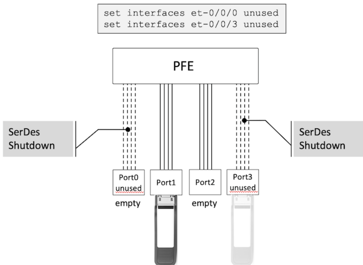
Figure 2: Configuring “Unused” Directly Connected Ports
