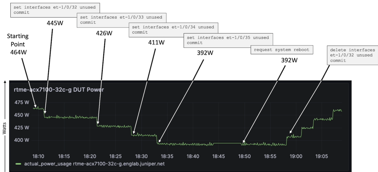
Figure 10: Impact of Reload for the 400GE Ports on ACX7100-32C
