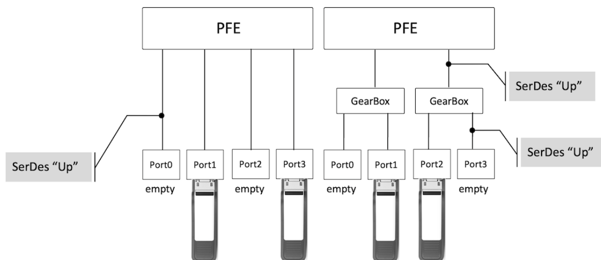
Figure 1: Default Behavior with Empty Ports on ACX7000
