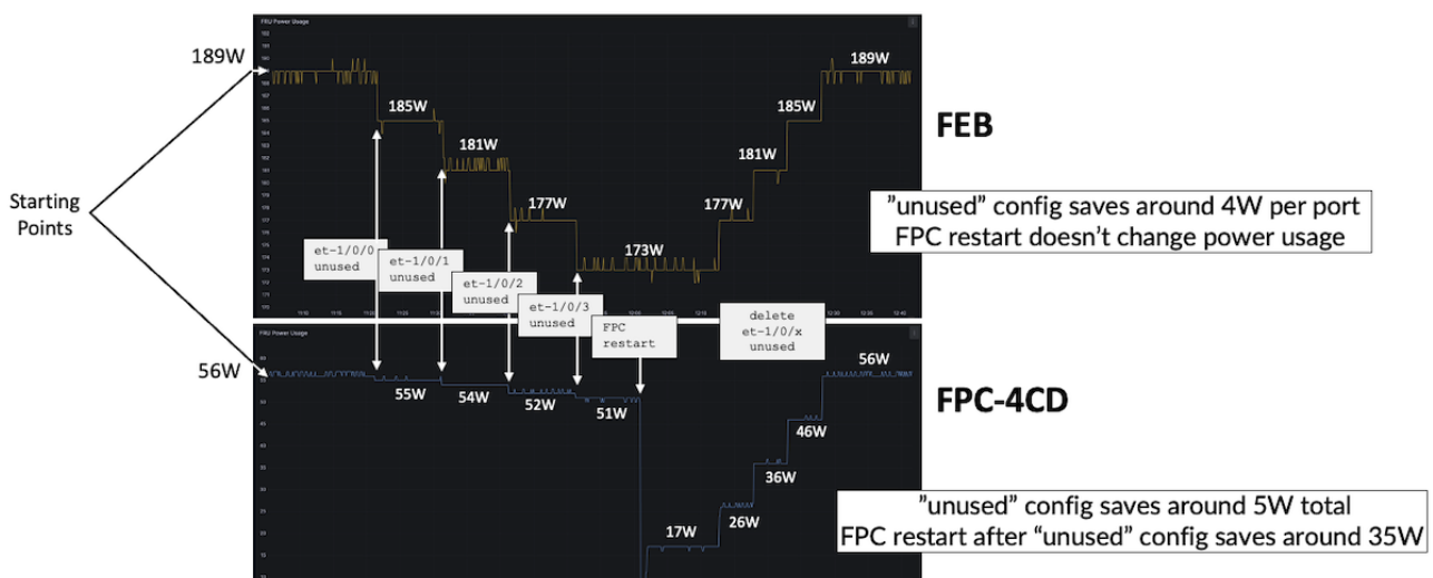
Figure 11: Power Saving Tests on ACX7509 with FPC-4CD
