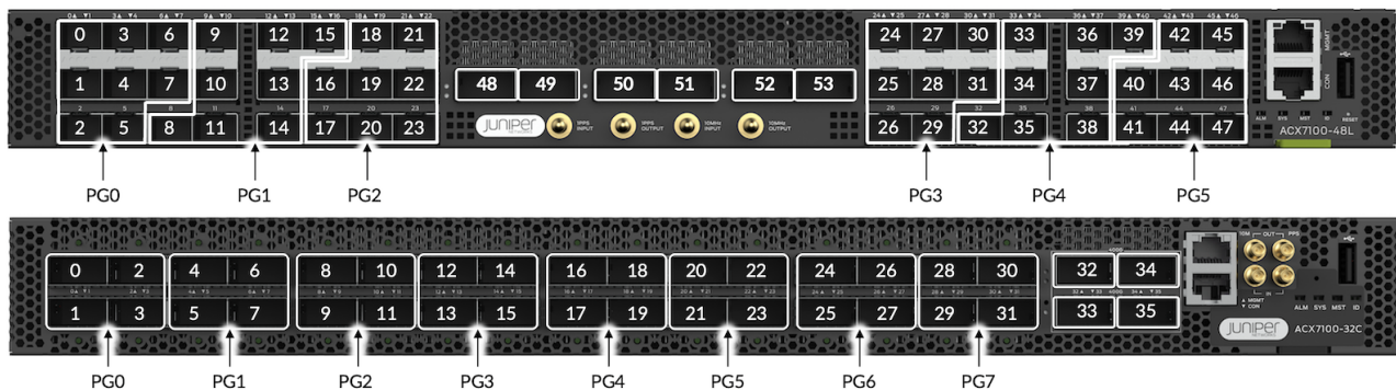
Figure 5: ACX7100 Ports Groups
