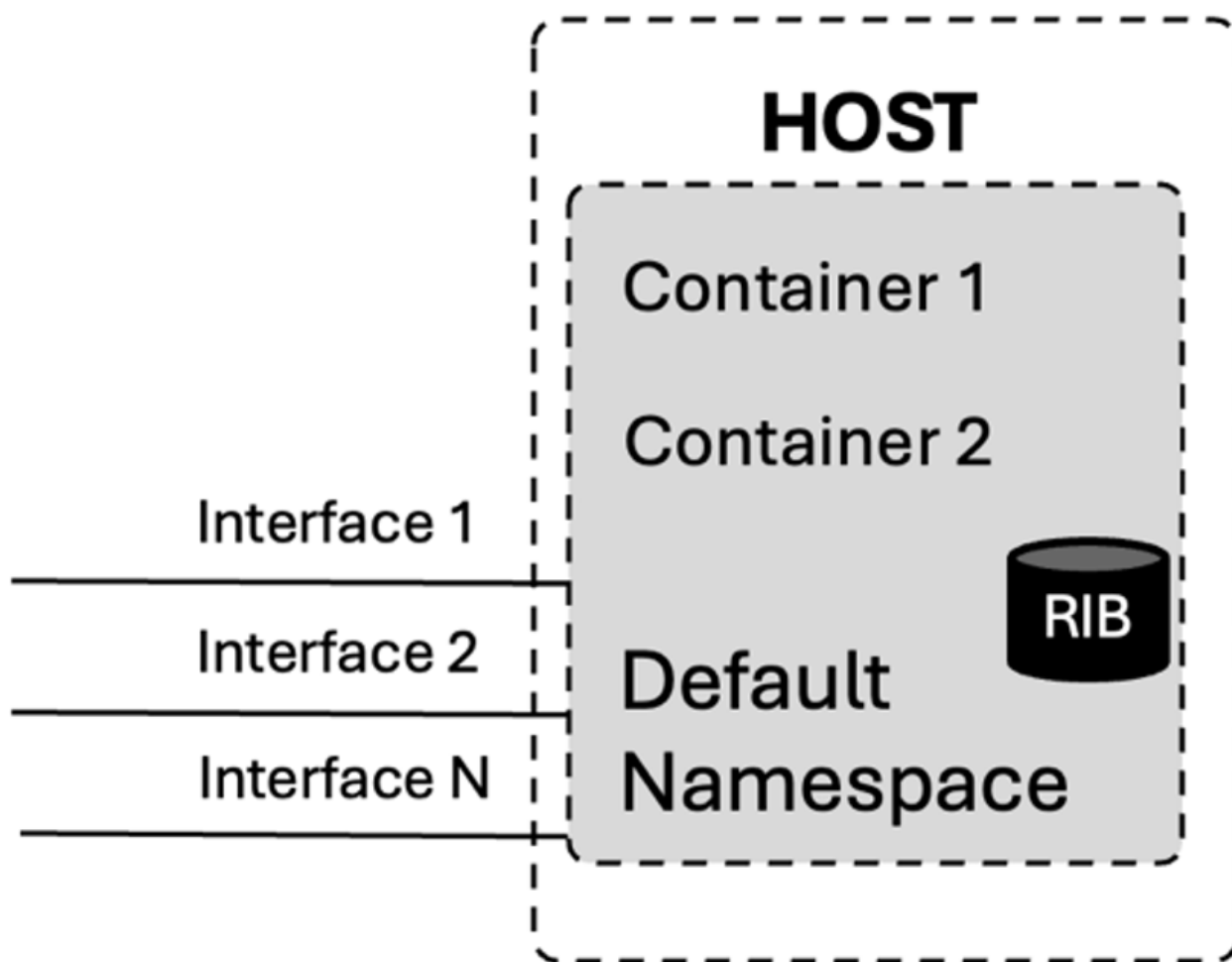
Figure 1: Containers in host mode
