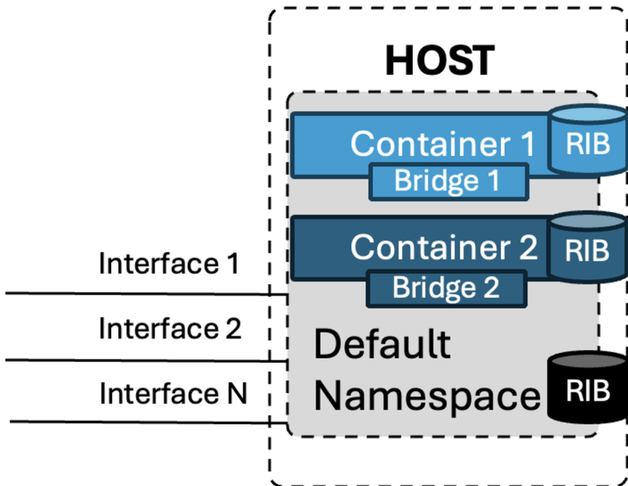
Figure 2: Containers in Bridge mode
