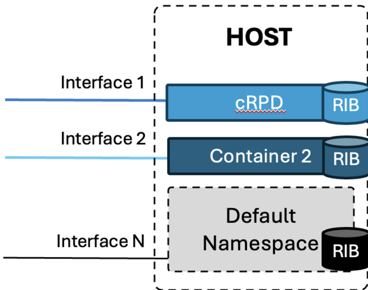
Figure 3: cRPD with separate resources
