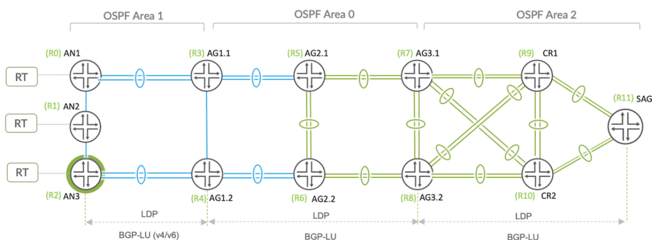
Figure 1: Lab Topology
