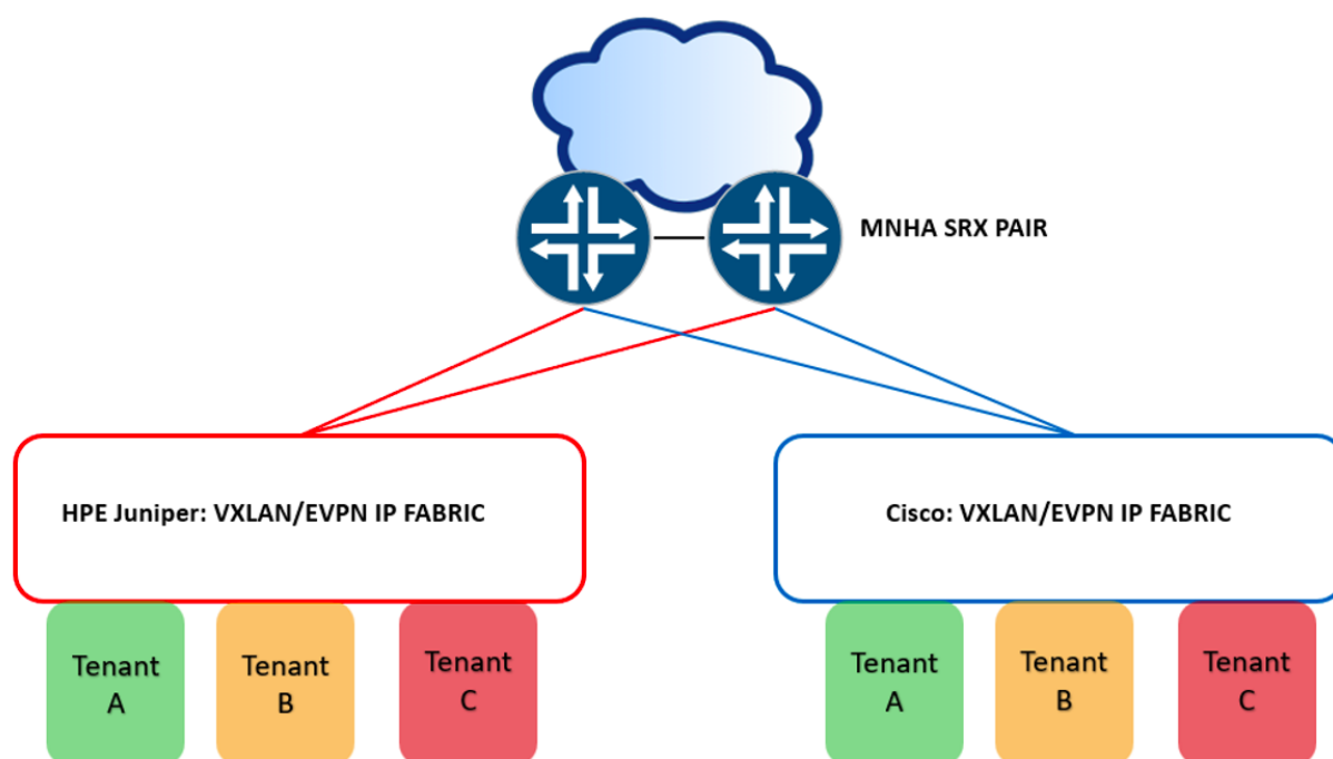
Figure 1: High Level Multi-Vendor Fabrics with MNHA
