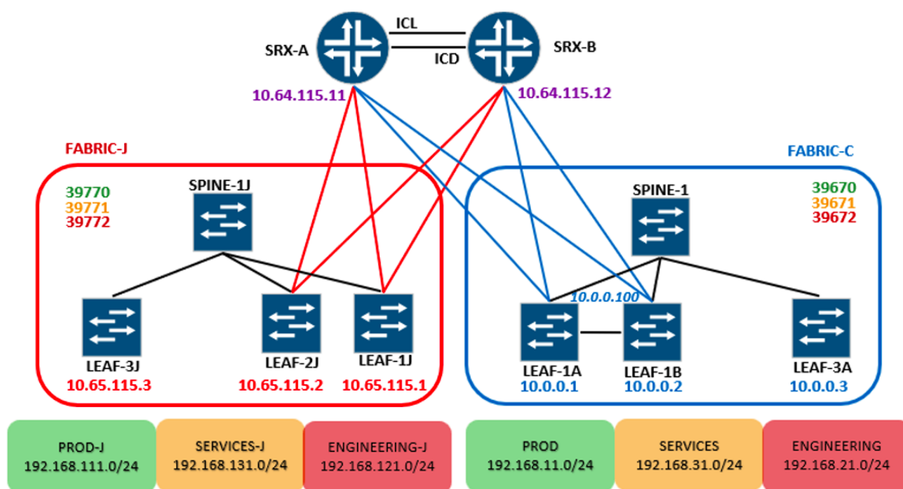
Figure 4: High Level SRX/Fabric/VNI/Tenant
