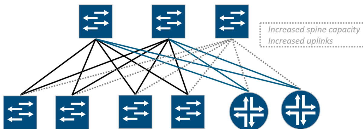
Figure 3: Spine Attached MNHA Pair
