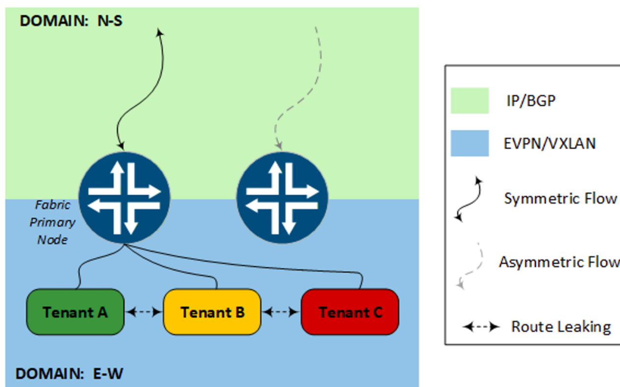
Figure 7: Single Fabric Primacy Domain View
