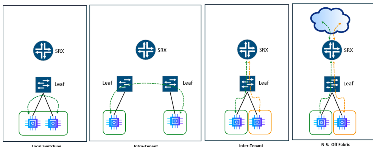
Figure 2: Forwarding Paths
