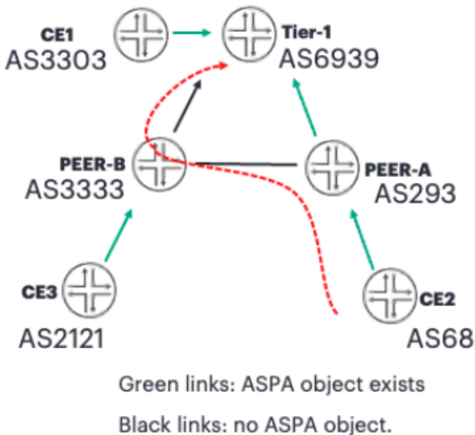
Figure 6: Leaking from AS3333 to an upstream
