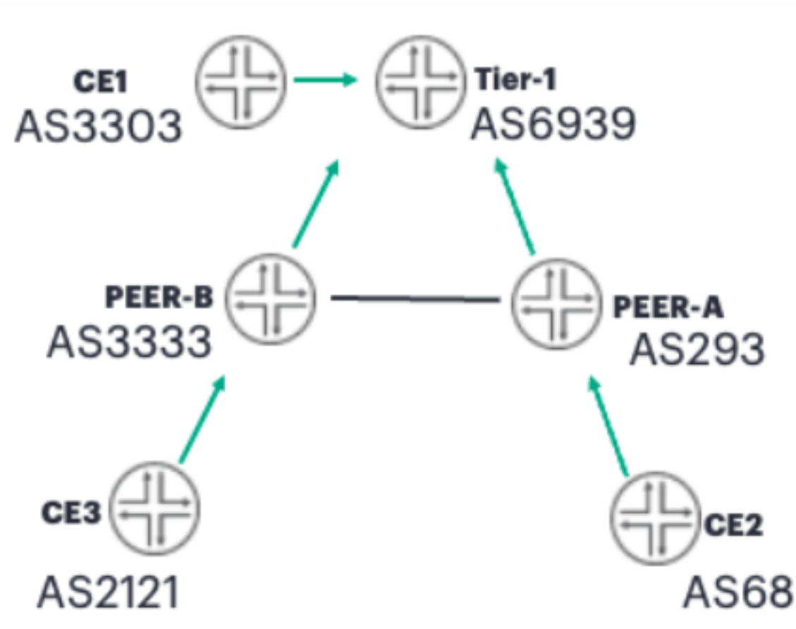
Figure 3: Reference Topology
