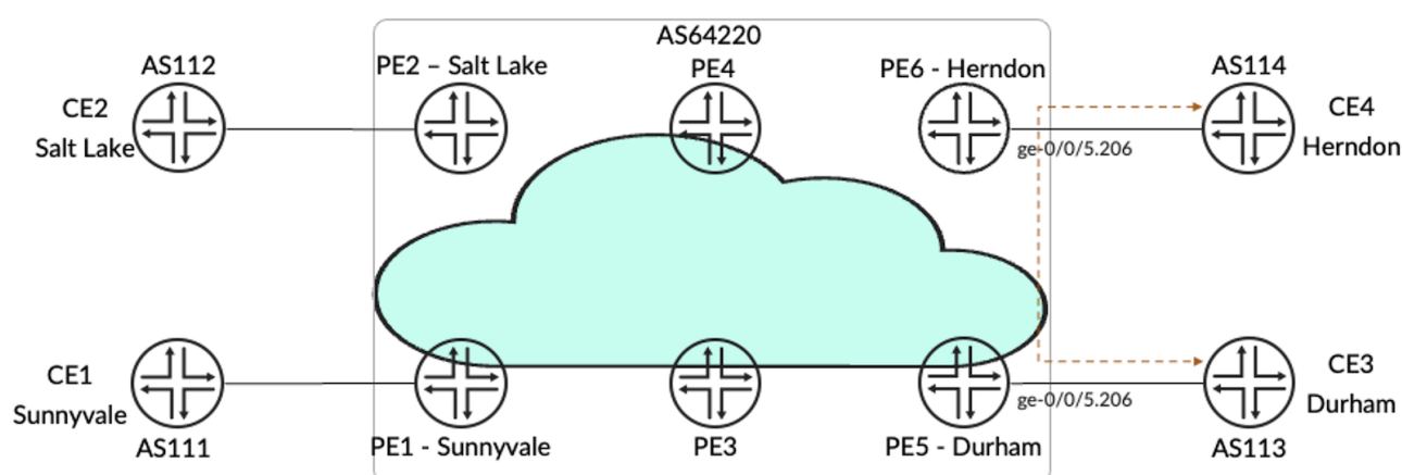
Figure 13: EVPN Topology
