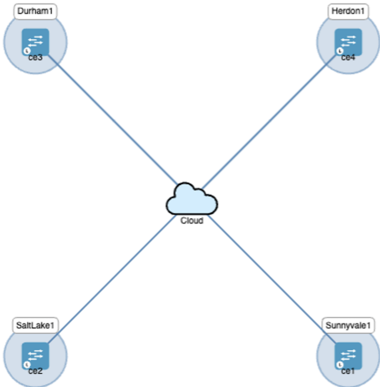
Figure 8: Service Topology of L3VPN (Any-to-any)
