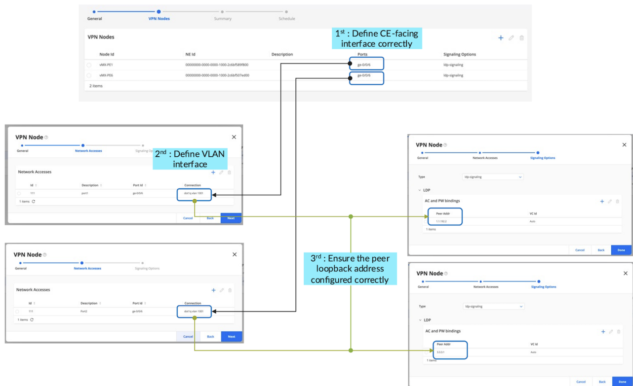
Figure 20: Step-by-step L2Circuit Service Provisioning from PA GUI
