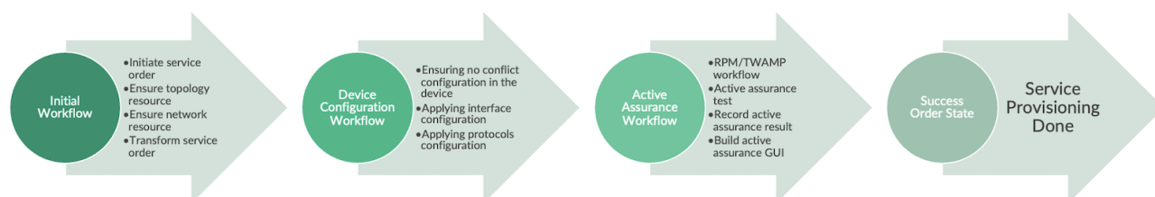
Figure 10: L3VPN High-Level Service Orchestration Workflow
