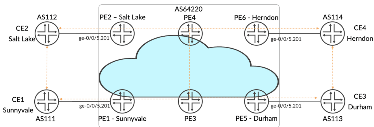
Figure 5: L3VPN Any-to-any topology
