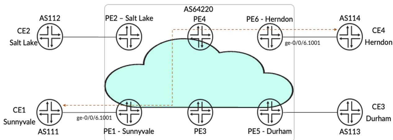
Figure 19: L2Circuit Topology
