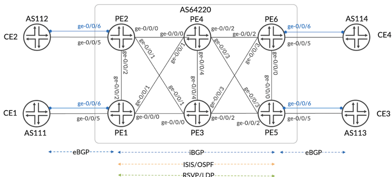
Figure 1: Network Topology
