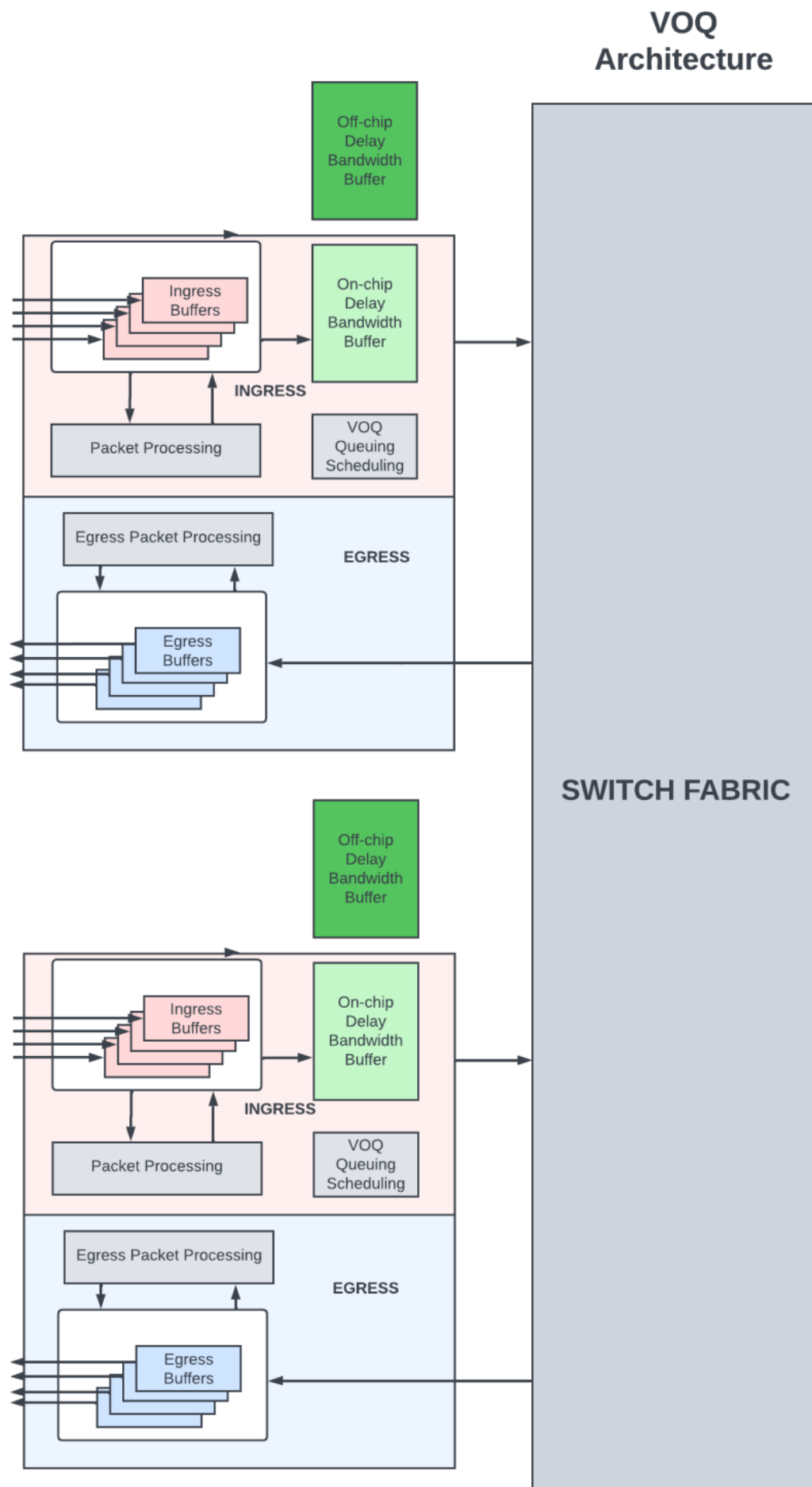
Figure 3: VOQ architecture
