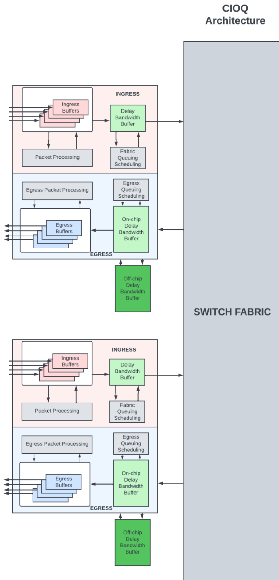
Figure 2: CIOQ architecture
