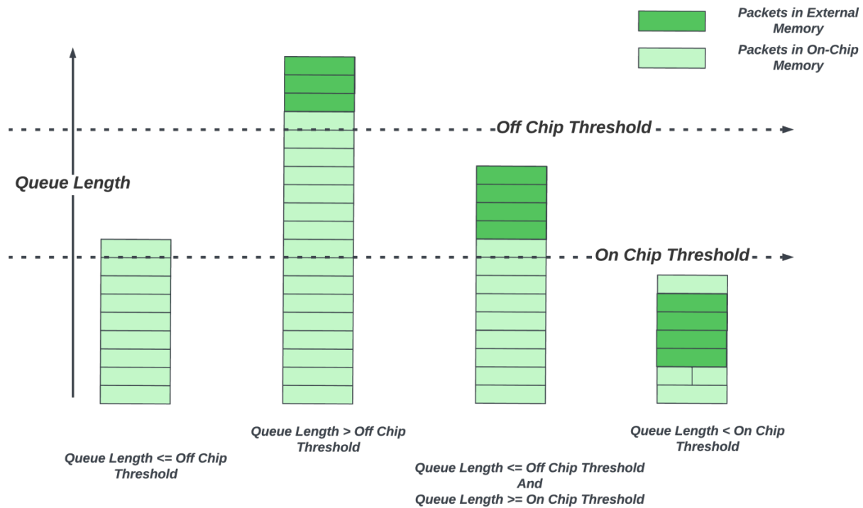
Figure 6: Hybrid buffering model
