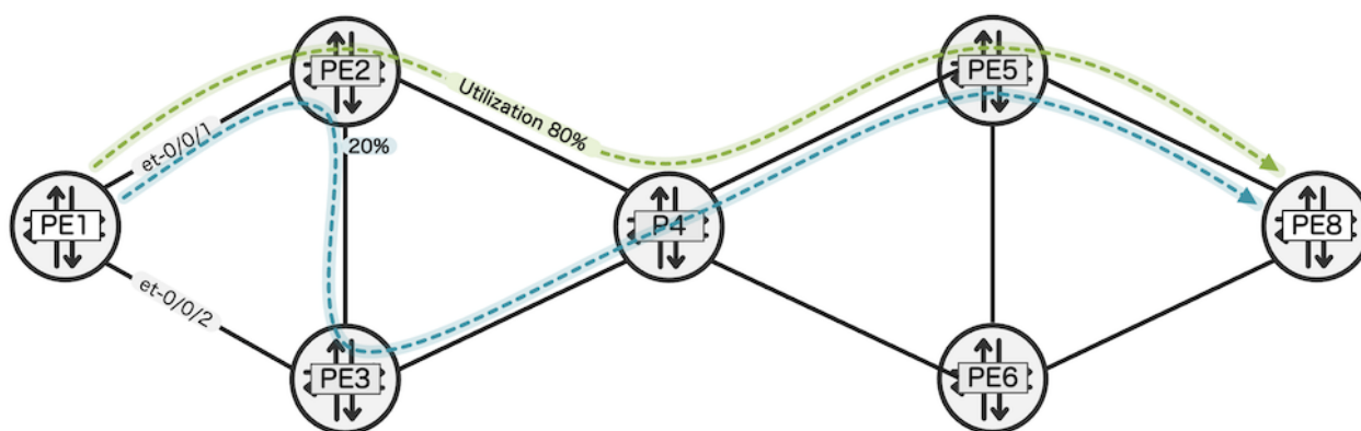
Figure 2: Congestion handled by the SR transit router with TTE
