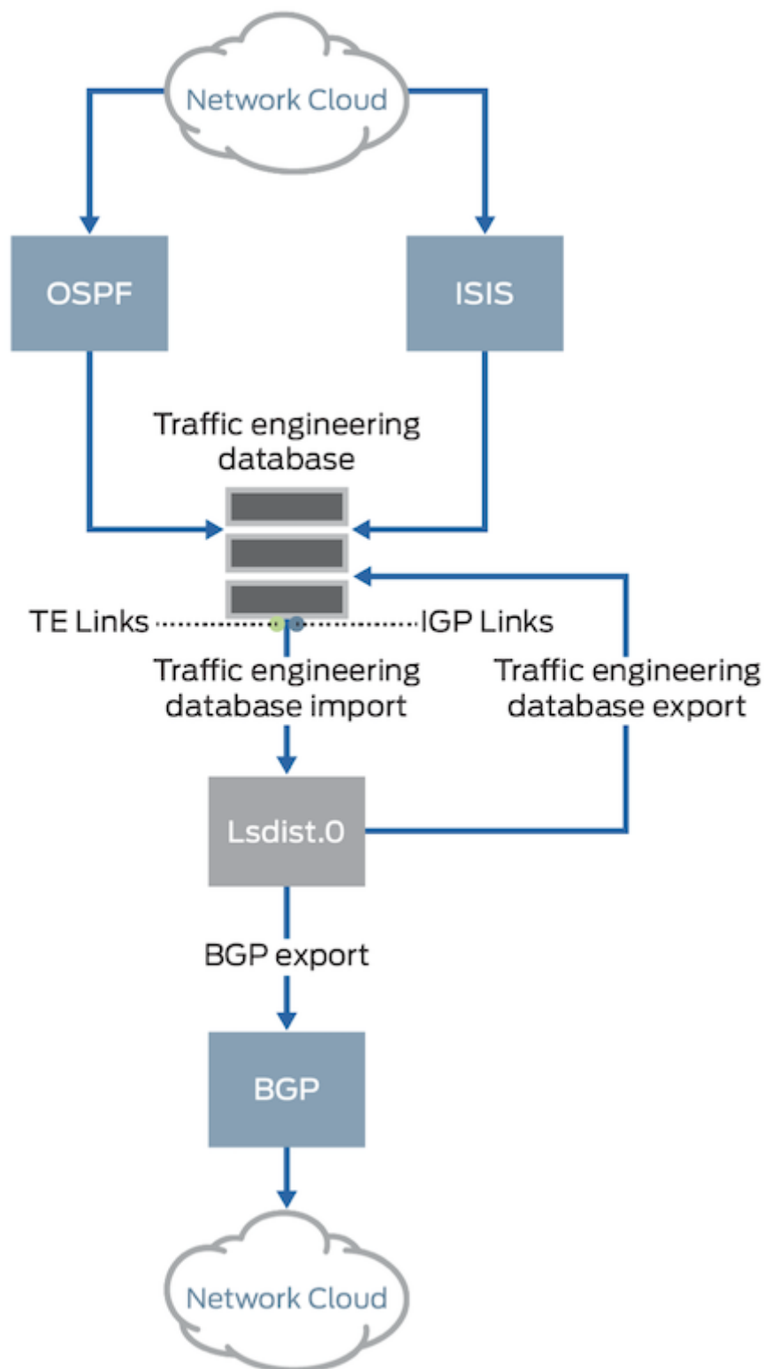
Figure 2: JUNOS Implementation of BGP Link-State Distribution
