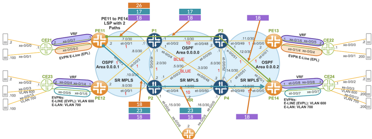
Figure 6: SR-TE LSP with DELAY Metric and Admin Groups CSPF
