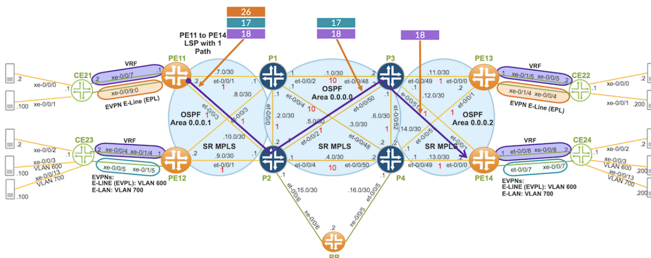
Figure 5: SR-TE LSP with DELAY Metric CSPF
