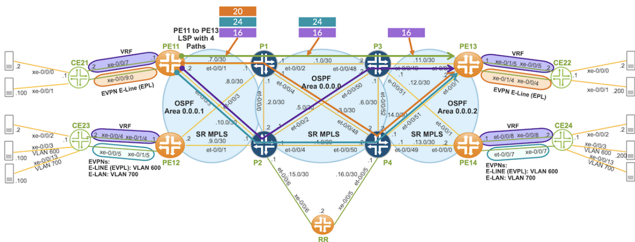
Figure 3: SR-TE LSP with IGP Metric CSPF
