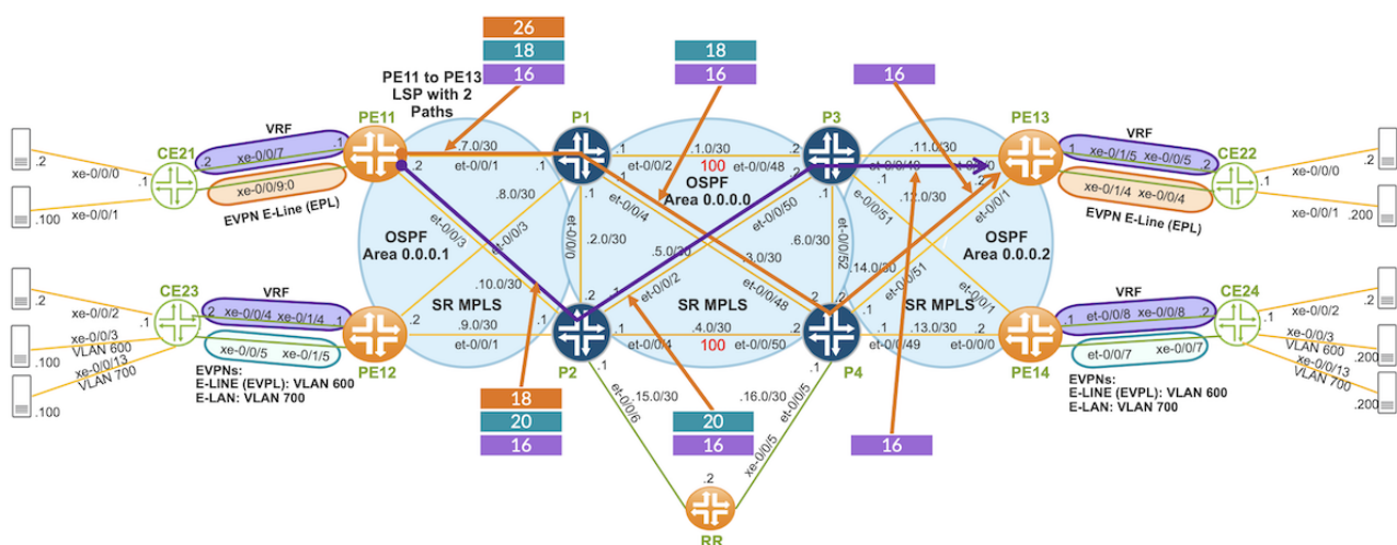
Figure 4: SR-TE LSP w/TE Metric CSPF
