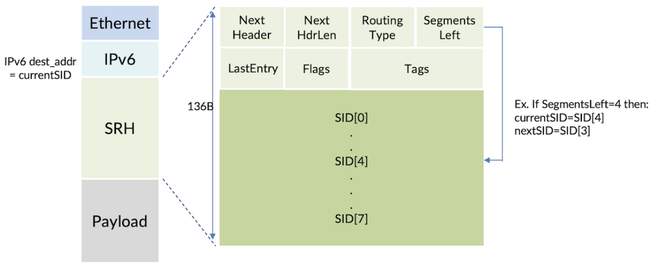
Figure 1: Segment Routing Header with 8 SIDs
