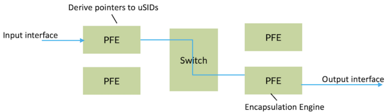
Figure 3: Passing Pointers
