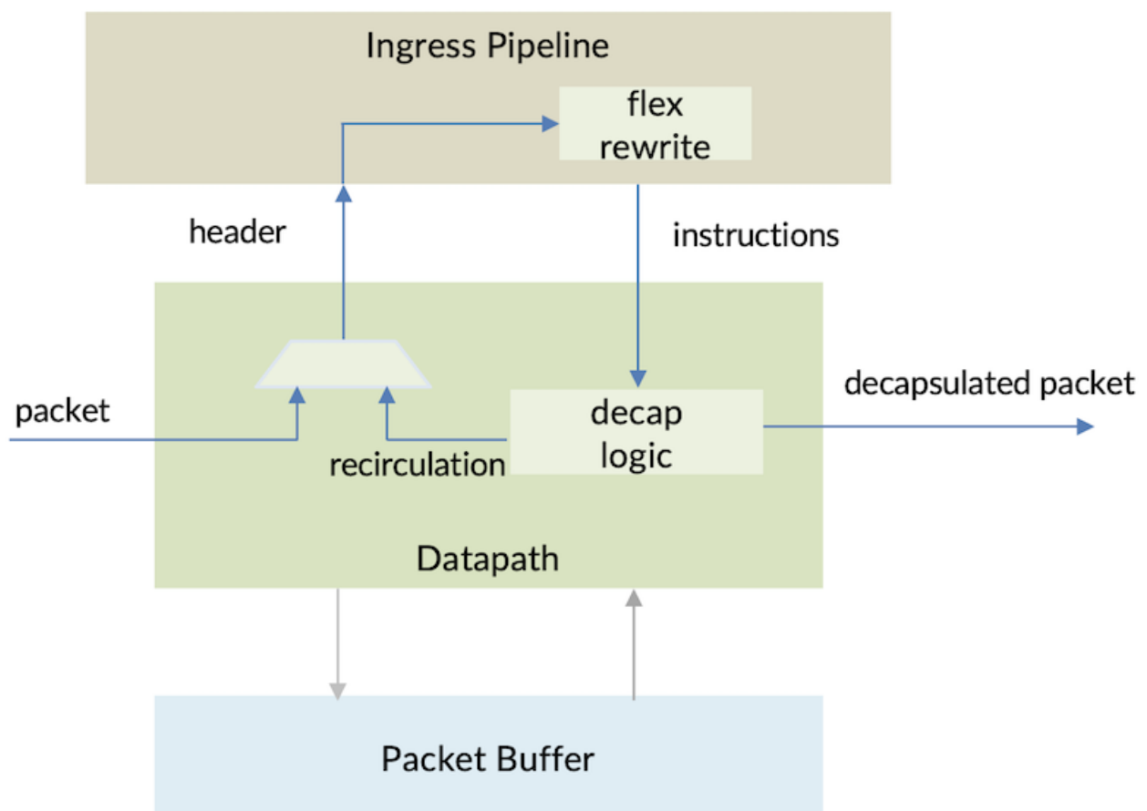
Figure 4: Packet Decapsulation and Recirculation in Datapath
