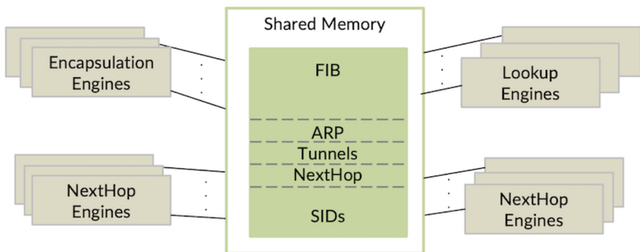
Figure 2: Shared Fungible On-Chip Memory
