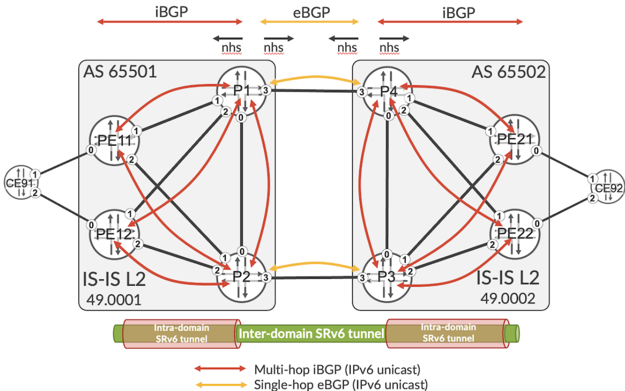
Figure 2 : Inter-AS Topology and transport prefix (loopbacks, SRv6 locators) distribution
