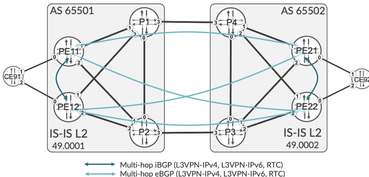
Figure 1: Inter-AS Topology and L3VPN service prefix distribution
