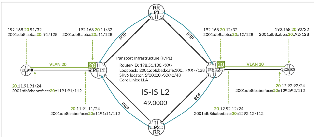
Figure 3: Basic SRv6 topology with L3VPN
