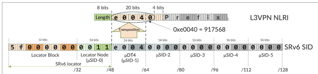
Figure 4: SRv6 Transposition
