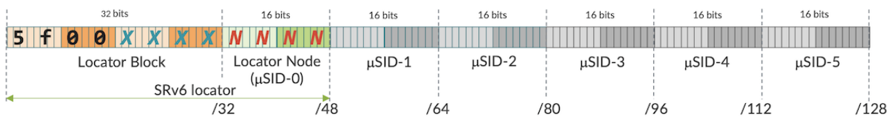
Figure 2: SRv6 Compressed SID Container
