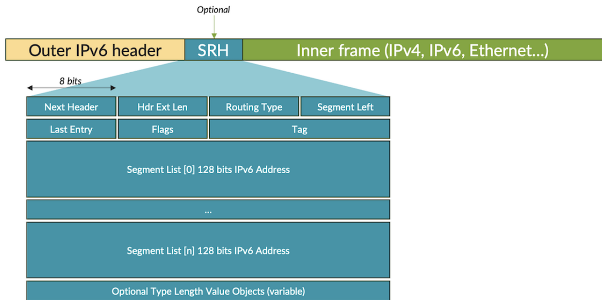
Figure 1: SRv6 Encapsulation Layers
