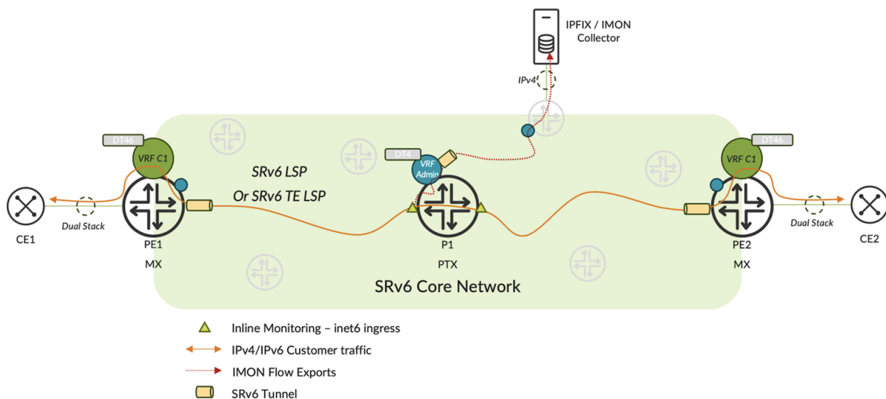
Figure 2: SRv6-Enabled Network
