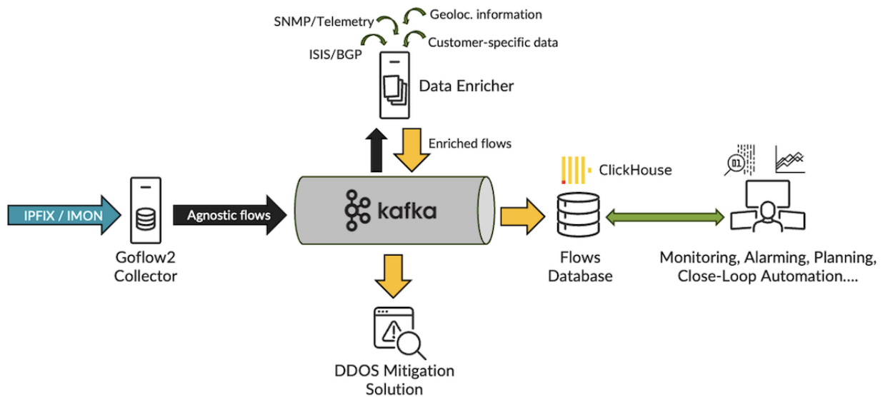
Figure 3: Typical OpenSource based solution for Flows management
