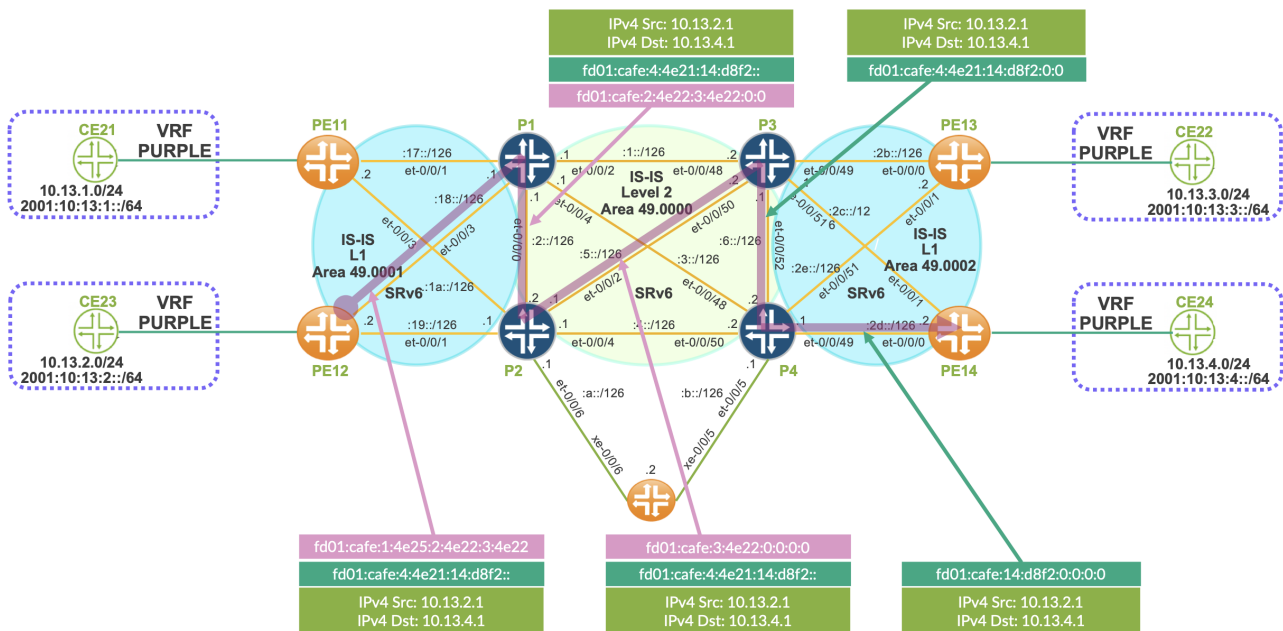
Figure 5: Static LSP using uN;uA segments
