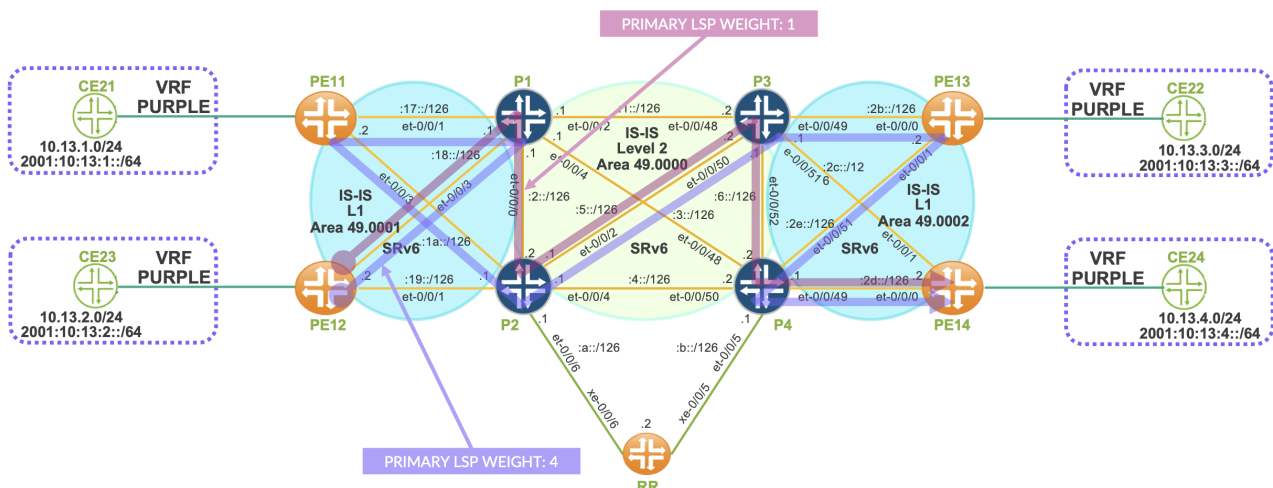
Figure 8: Static LSP with Weighted Load Balancing
