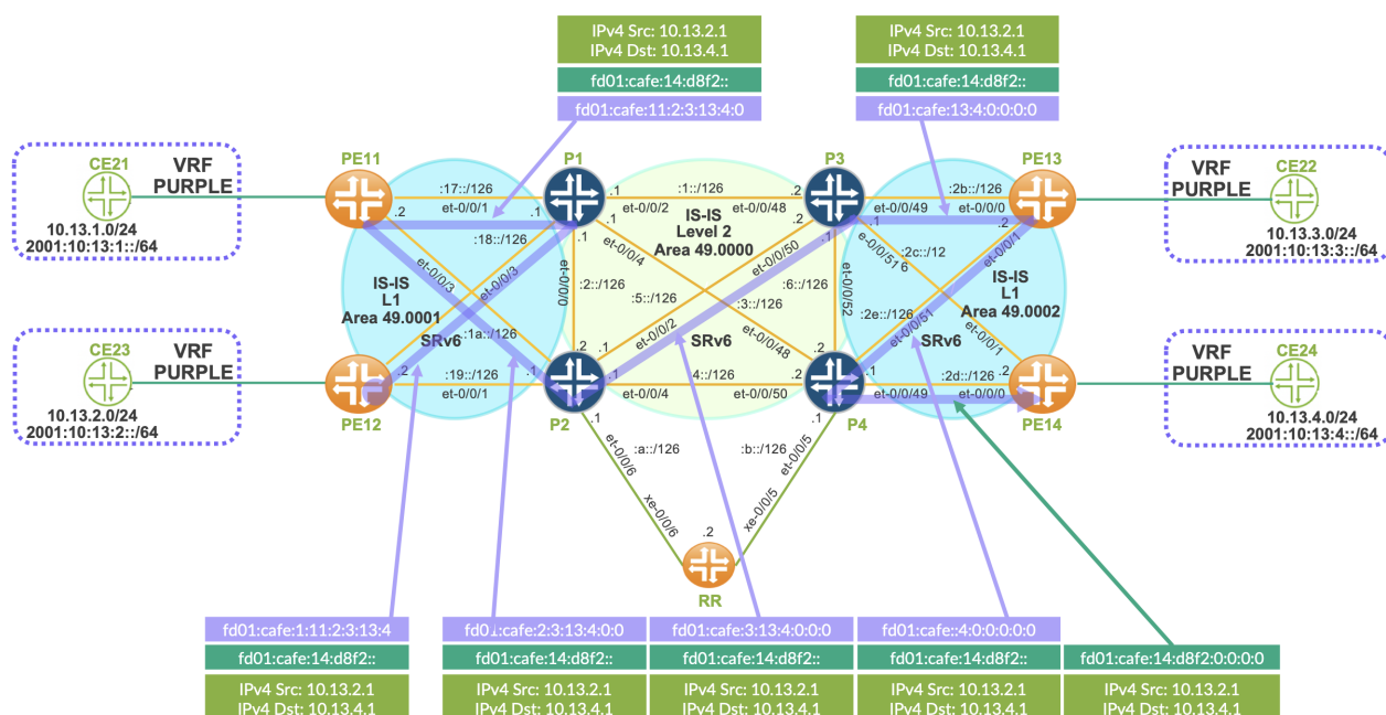
Figure 2: Static LSP using uN segments
