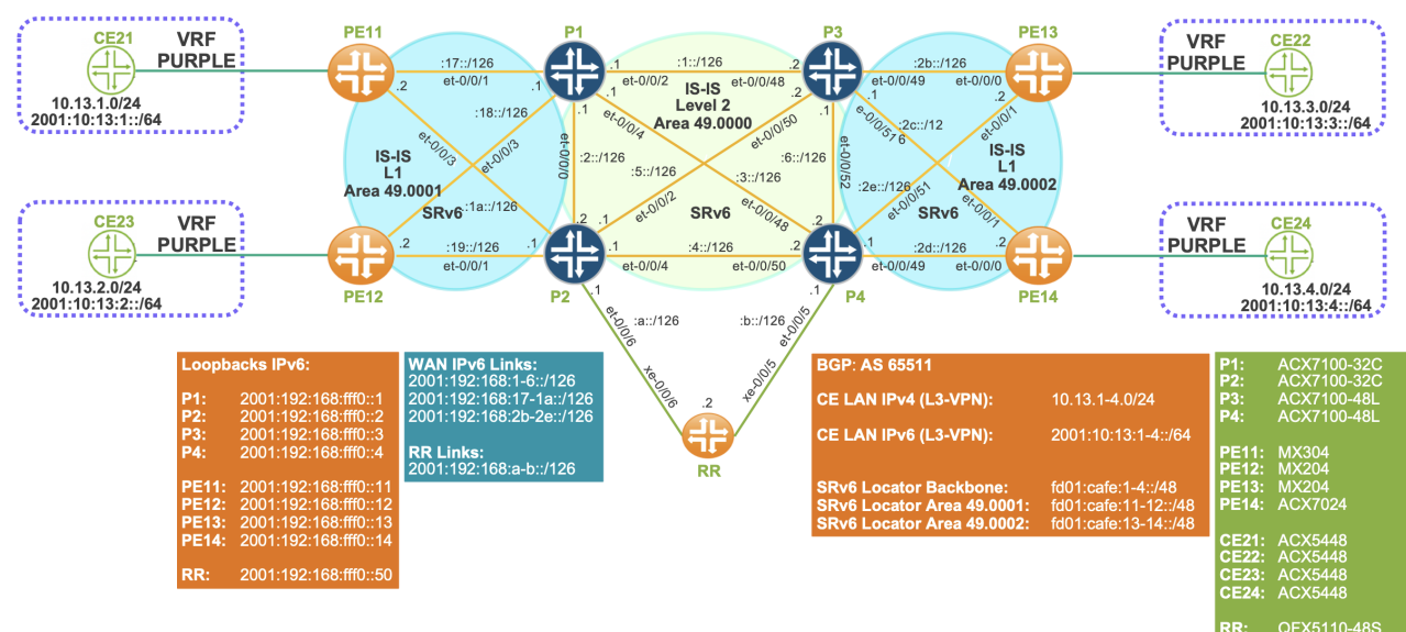
Figure 1: Multi-Domain IS-IS Network
