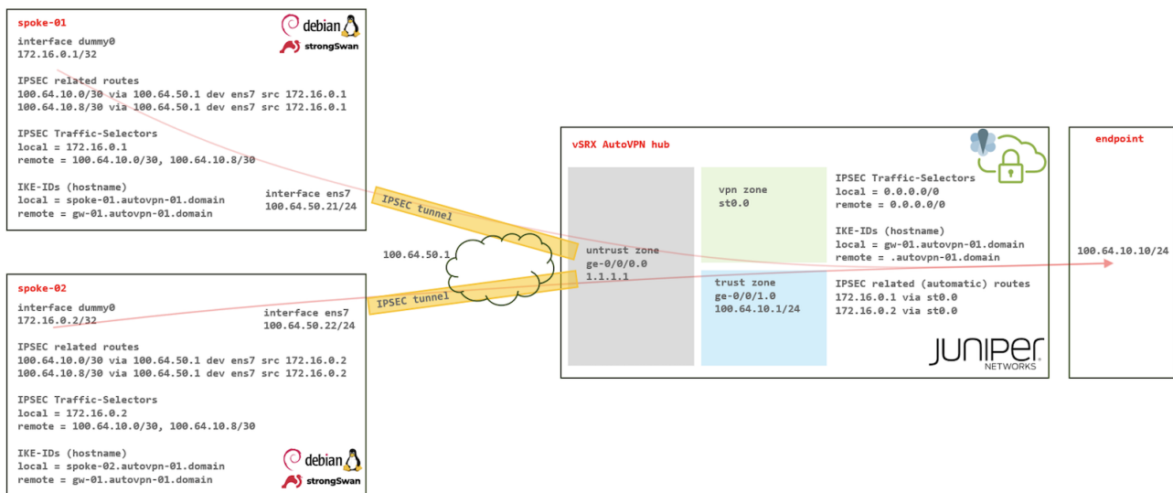
Figure 1: Demo Linux - SRX AutoVPN topology
