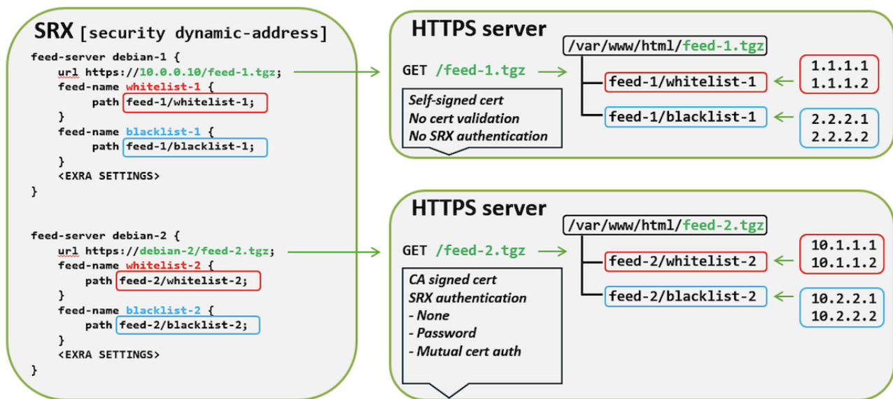
Figure 3: Features of the two feed-servers
