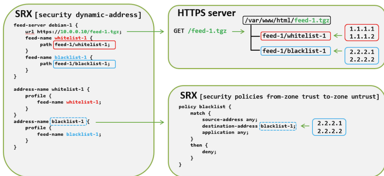
Figure 2: SRX configuration / feed-server contents relationship
