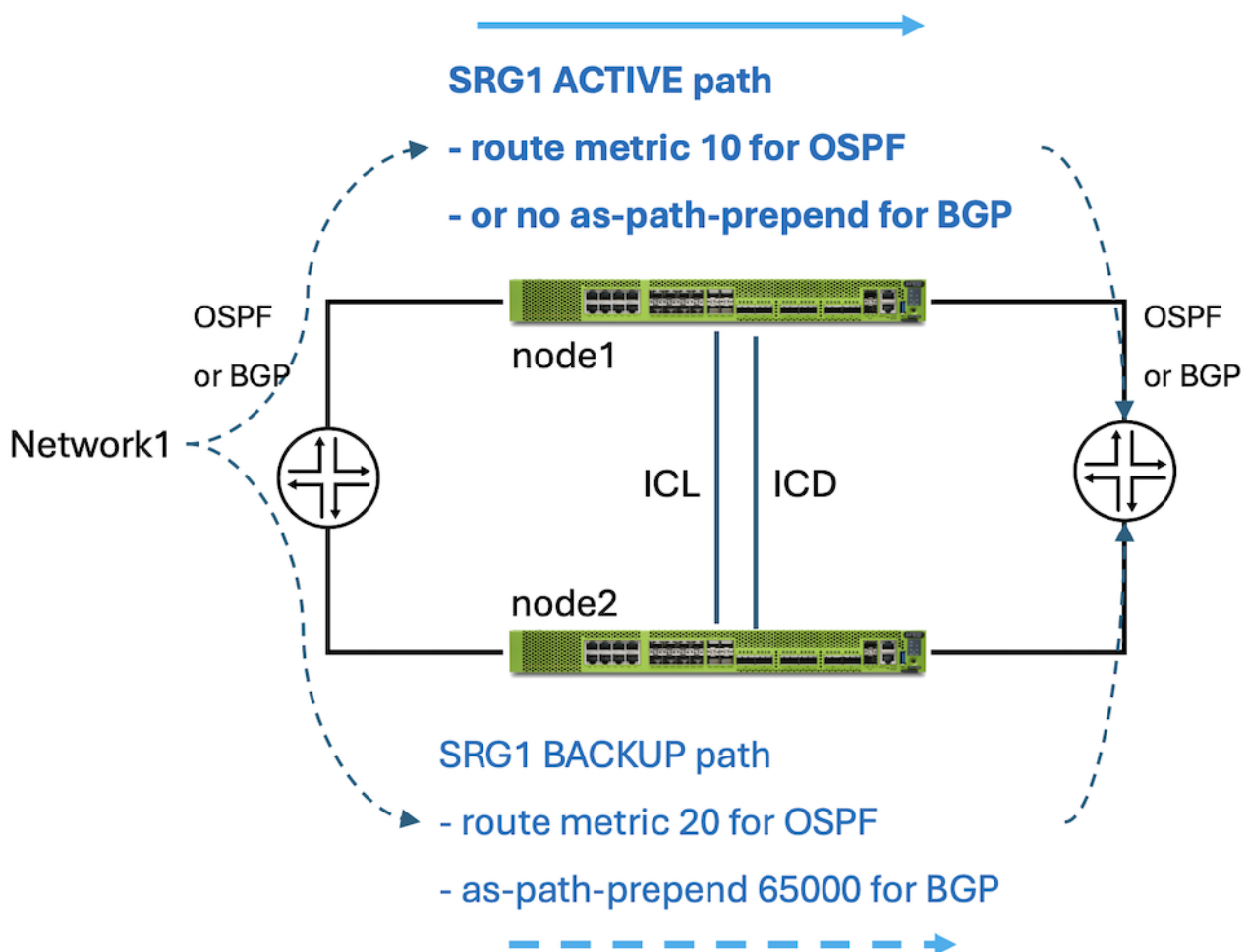
Figure 9: SRG1/SRG2 Active/Backup Options
