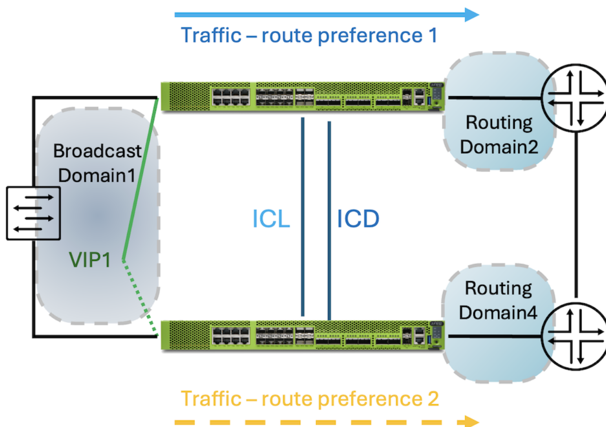
Figure 5: MNHA Hybrid Mode (L2-L3)
