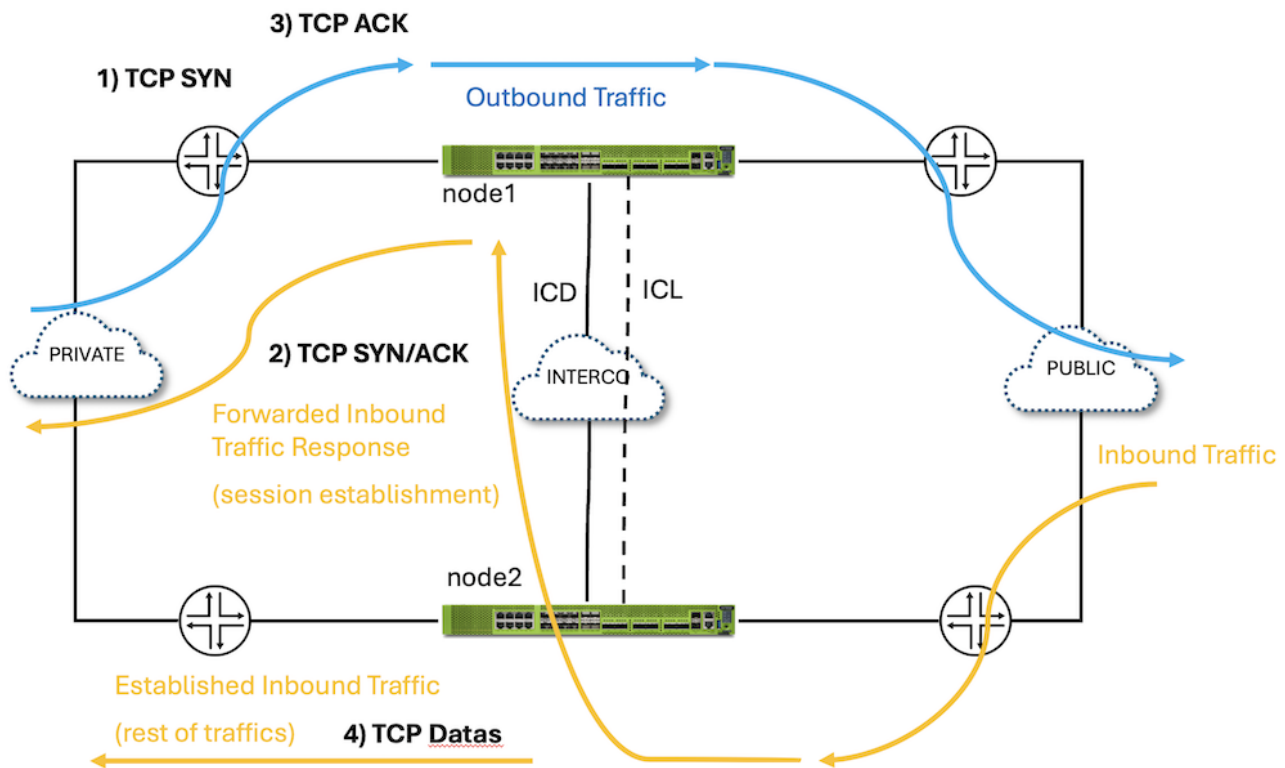
Figure 8: Asymmetric Traffic Flow
