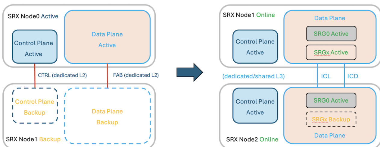
Figure 3: Chassis Cluster and MNHA internal structure
