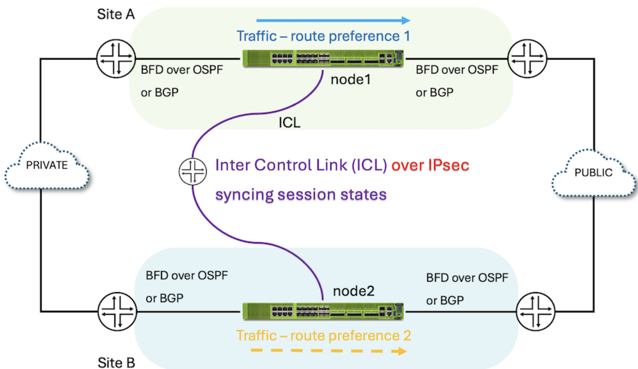
Figure 11: Distributed/Geo redundancy scenario
