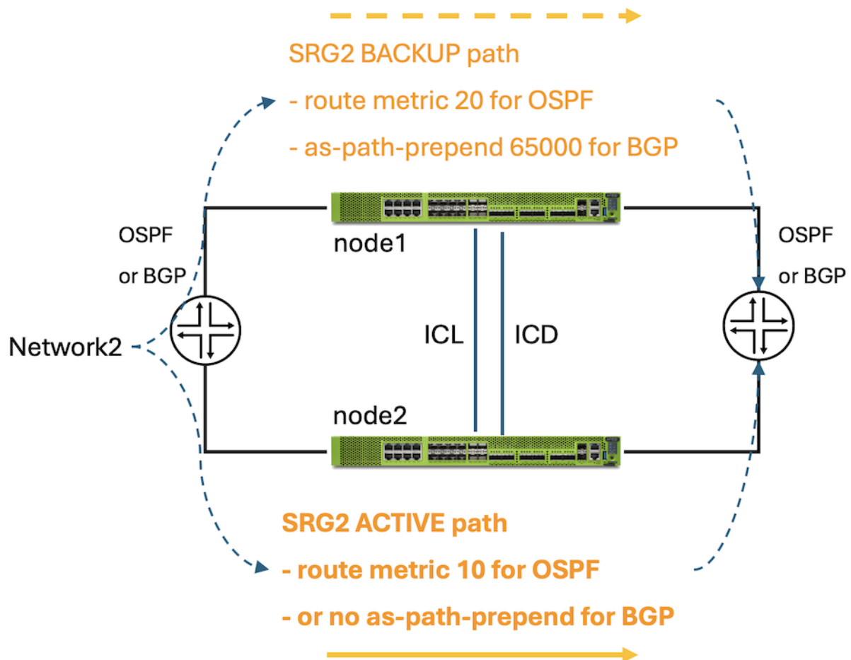
Figure 10: SRG1/SRG2 Active/Backup Options
