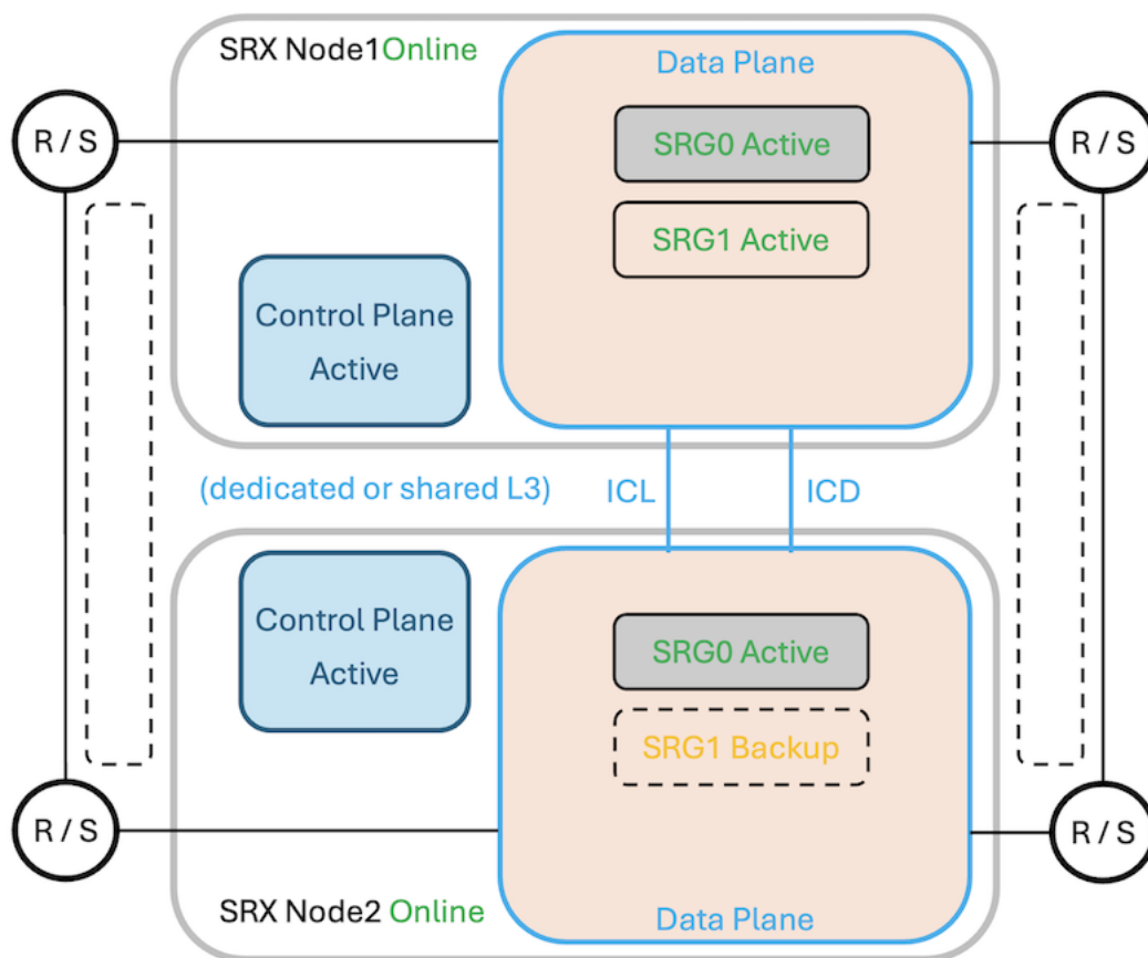
Figure 2: MNHA architecture of 2 nodes
