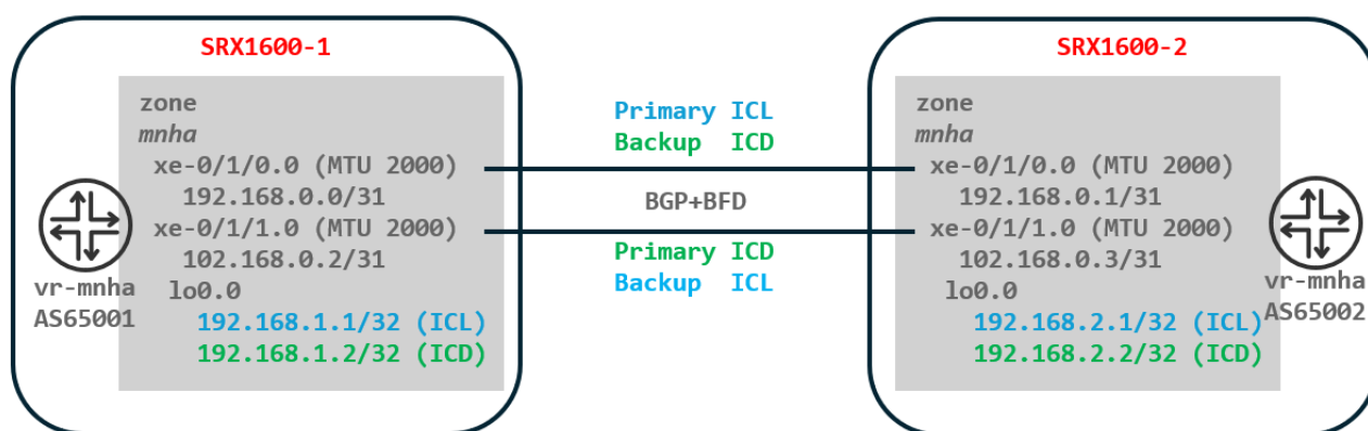
Figure 3: MNHA ICL and ICD links topology
