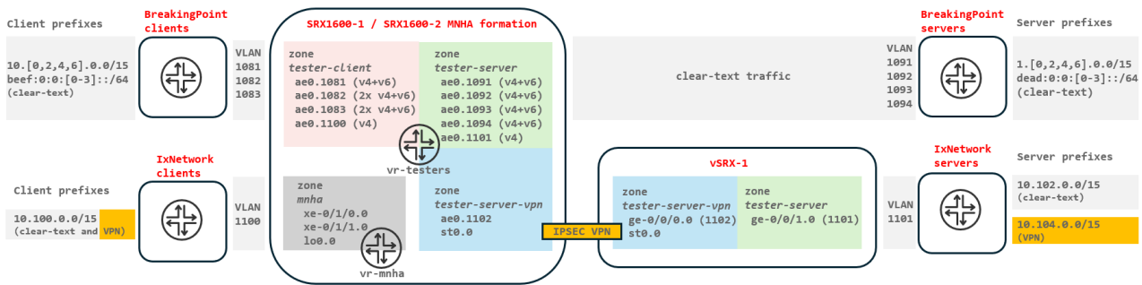
Figure 2: Simplified topology diagram
