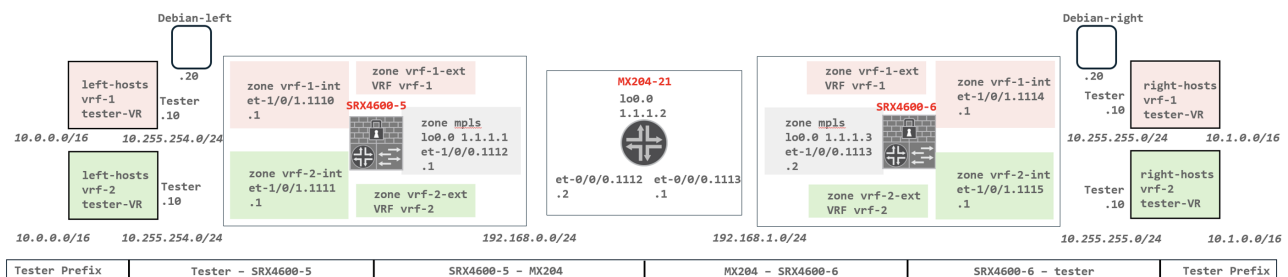
Figure 1: Demo topology
