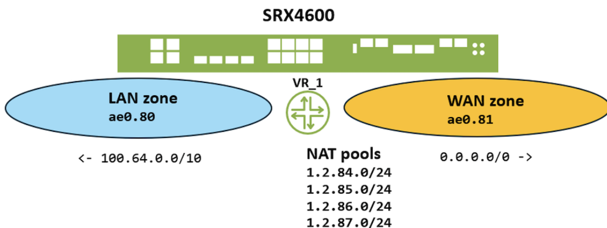
Figure 2: simplified SRX4600 setup layout
