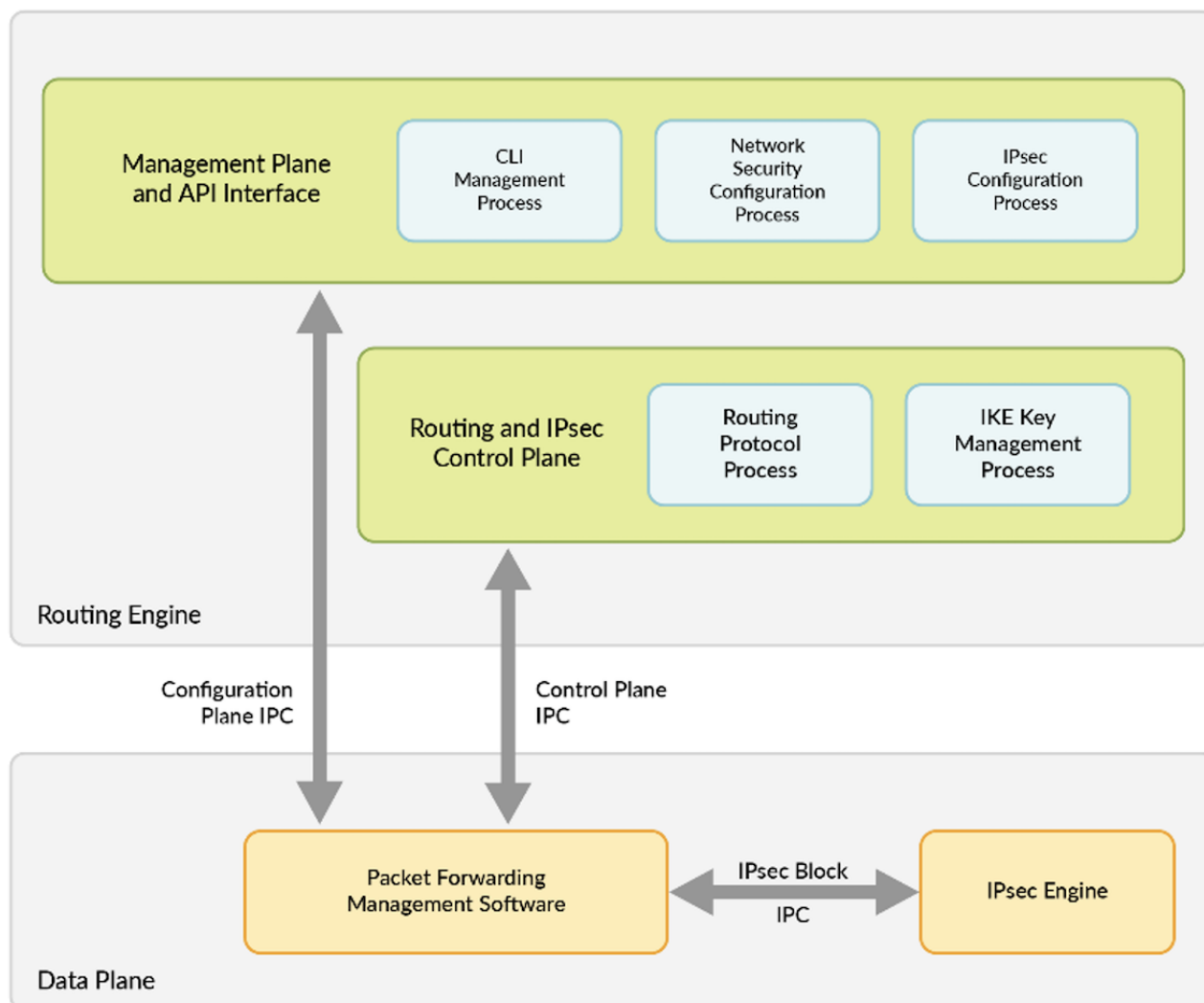
Figure 2: Generic block schema of inline-IPSEC architecture from Juniper documentation
