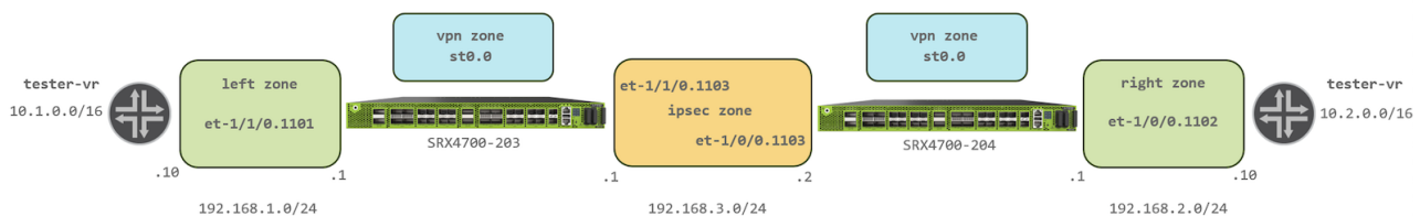
Figure 3: Logical topology schema
