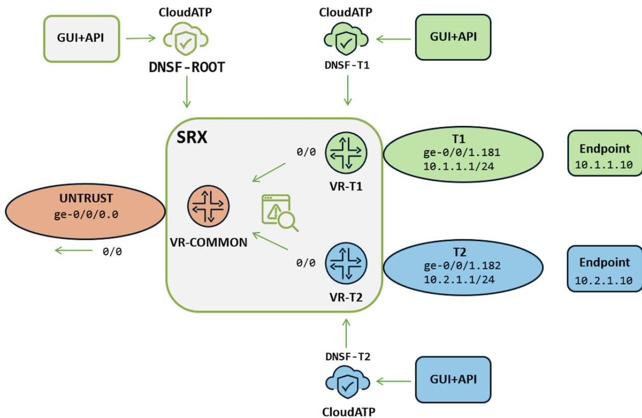
Figure 1: demo setup topology
