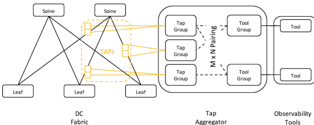
Figure 1: High Level View of the TAP Aggregation Solution
