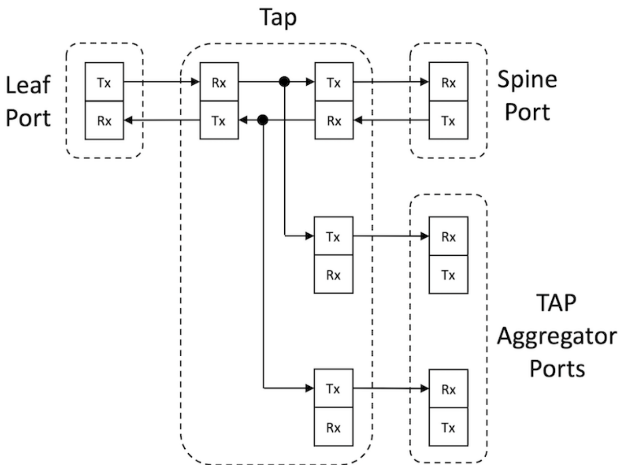
Figure 2: internal view of a TAP device to monitor a single bidirectional link
