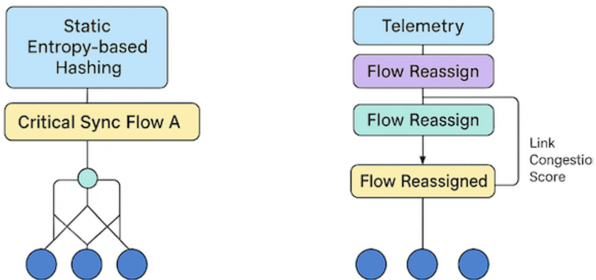
Figure 5: Entropy-aware ECMP
