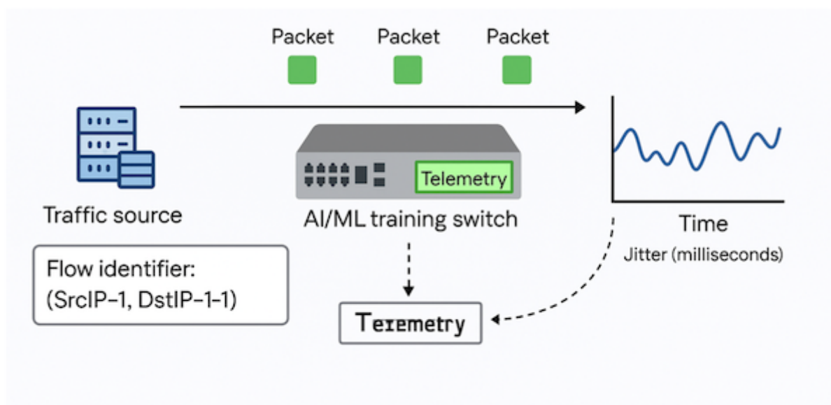
Figure 4: A modern jitter-aware telemetry stack segments flows
