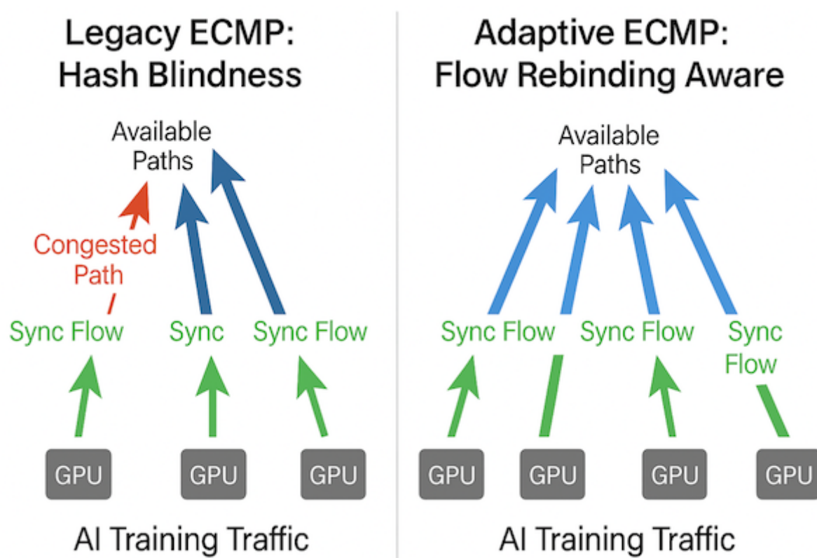
Figure 2: ECMP hash-based distribution
