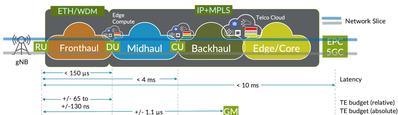
Figure 1: Synchronisation network topology
