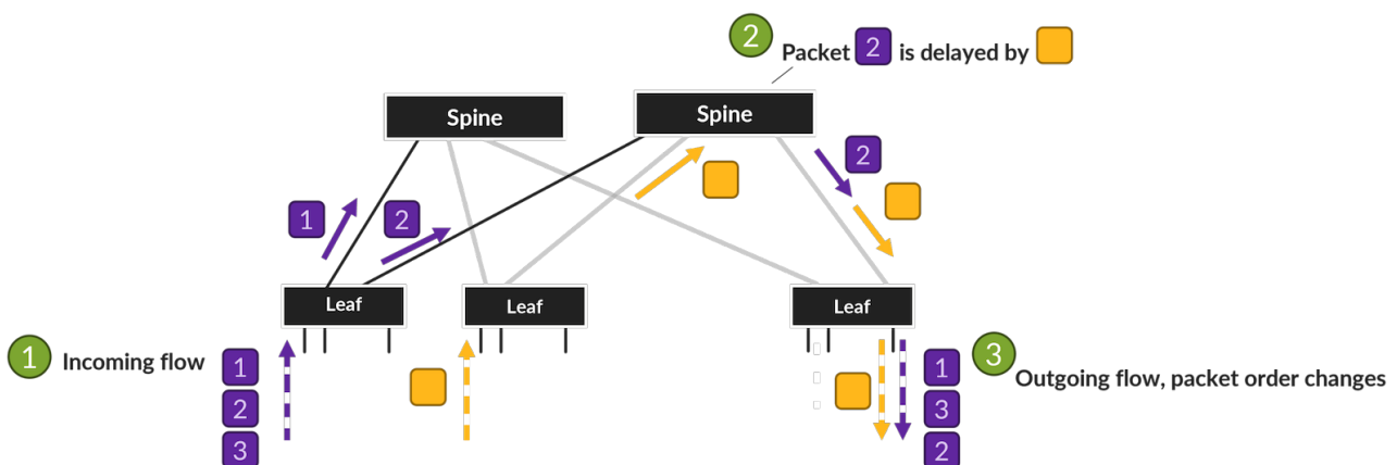
Figure 4: packet is delayed because of some other packet in the spine port queue
