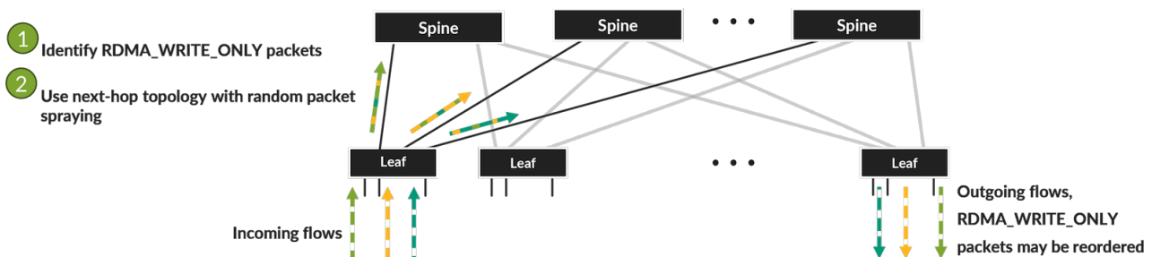
Figure 3: concept of the packet spraying solution
