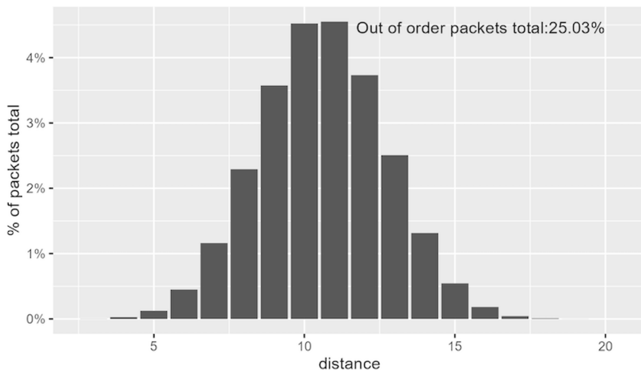
Figure 6: distance distribution of the packets
