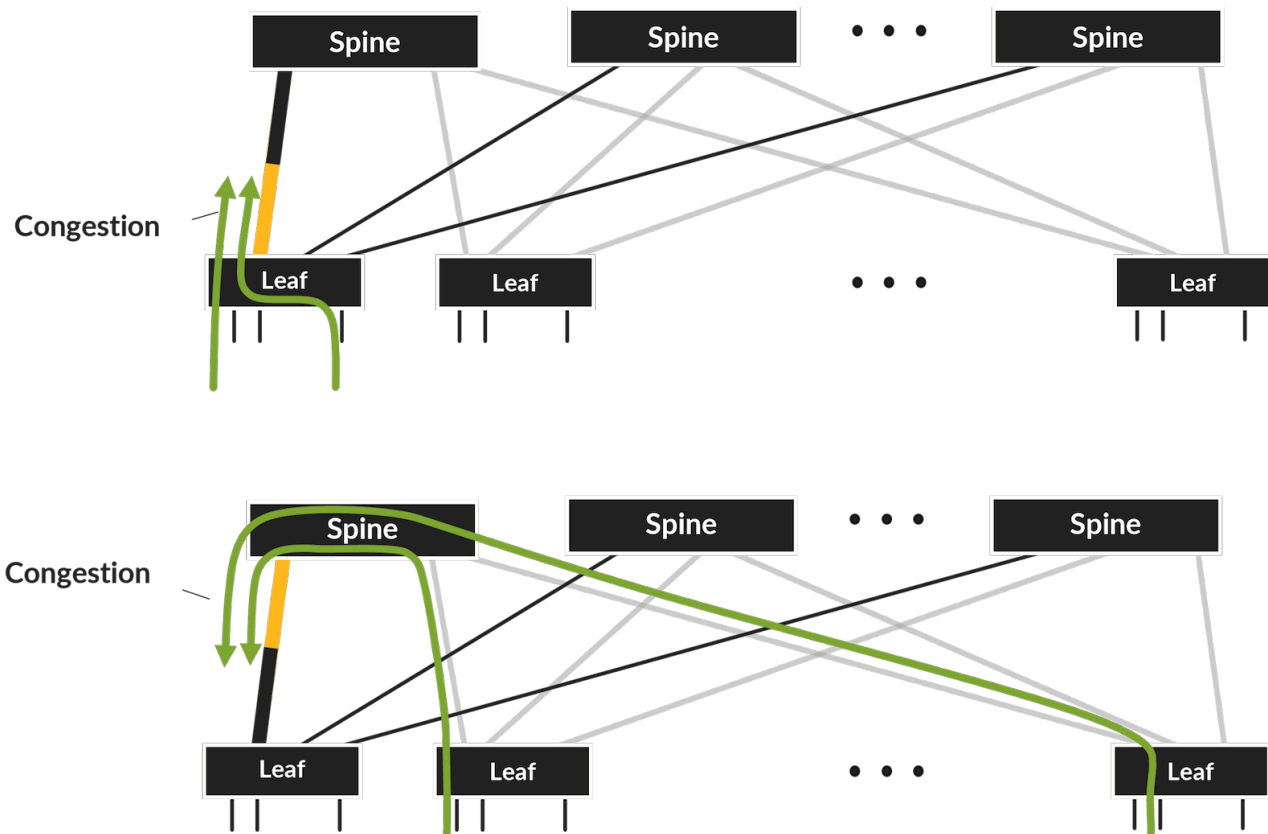
Figure 1: Typical fabric congestion points
