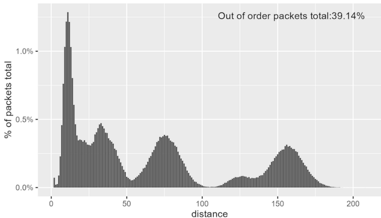
Figure 8: The resulting distance distribution
