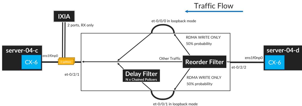
Figure 7: traffic flow through the router
