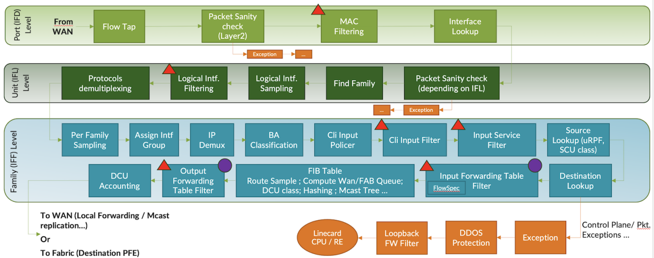
Figure 4: LUSS Packet Processing by Ingress PFE
