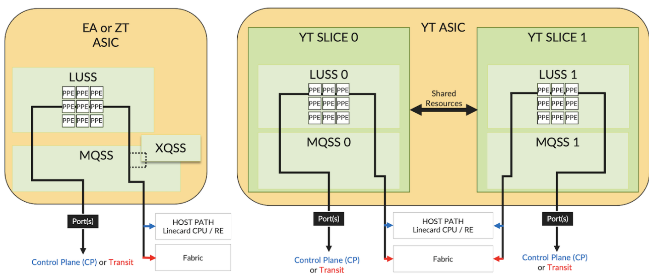
Figure 3: Simplified View of TRIO ASIC Architecture
