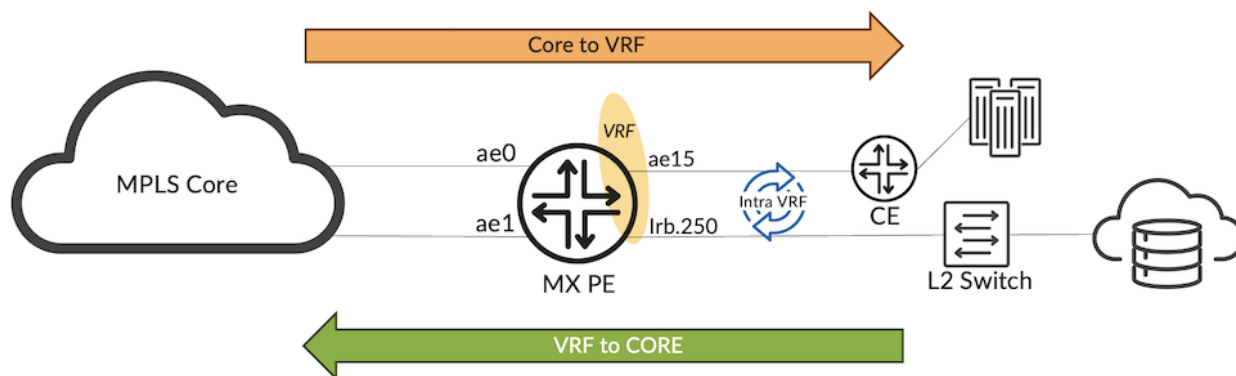
Figure 10: Per VRF Accounting Topology
