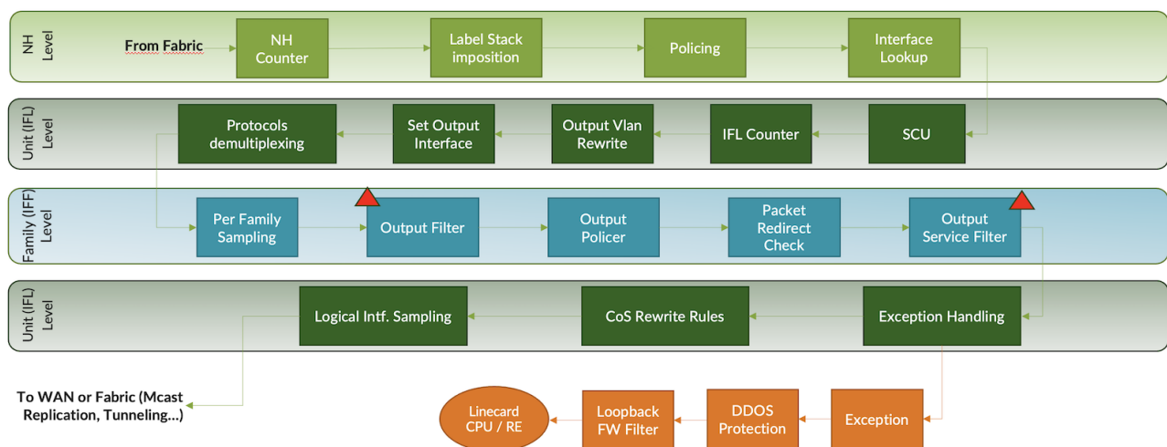
Figure 5: LUSS Packet Processing by Egress PFE
