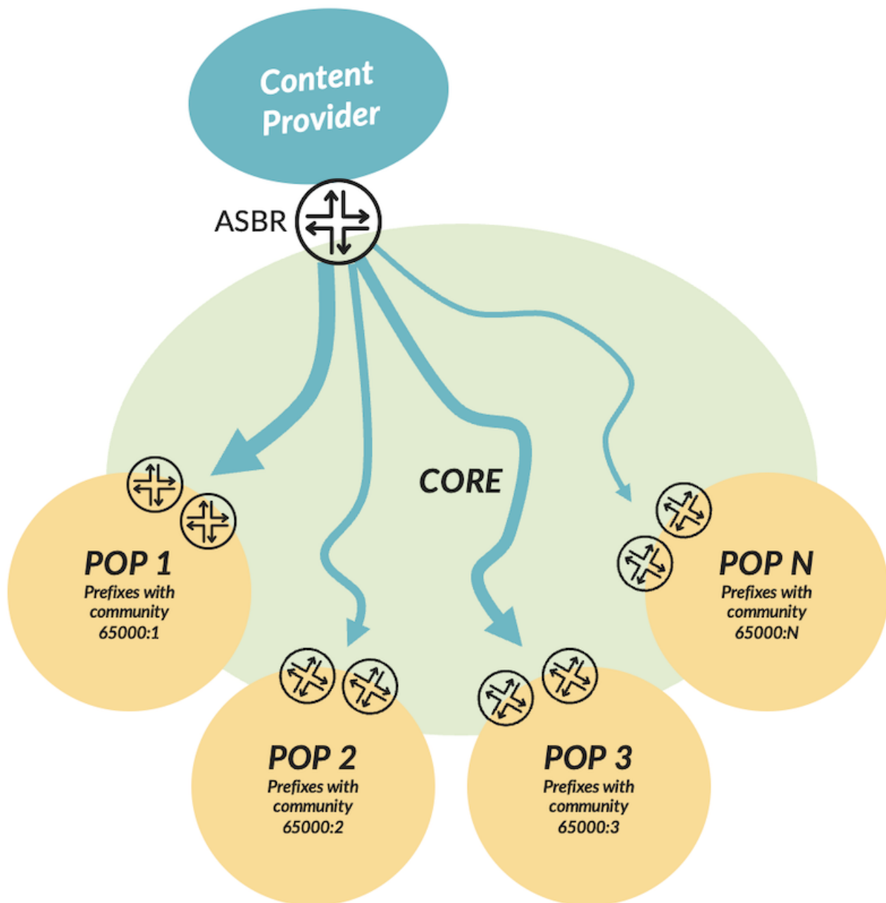
Figure 9: Per POP Traffic Distribution Topology
