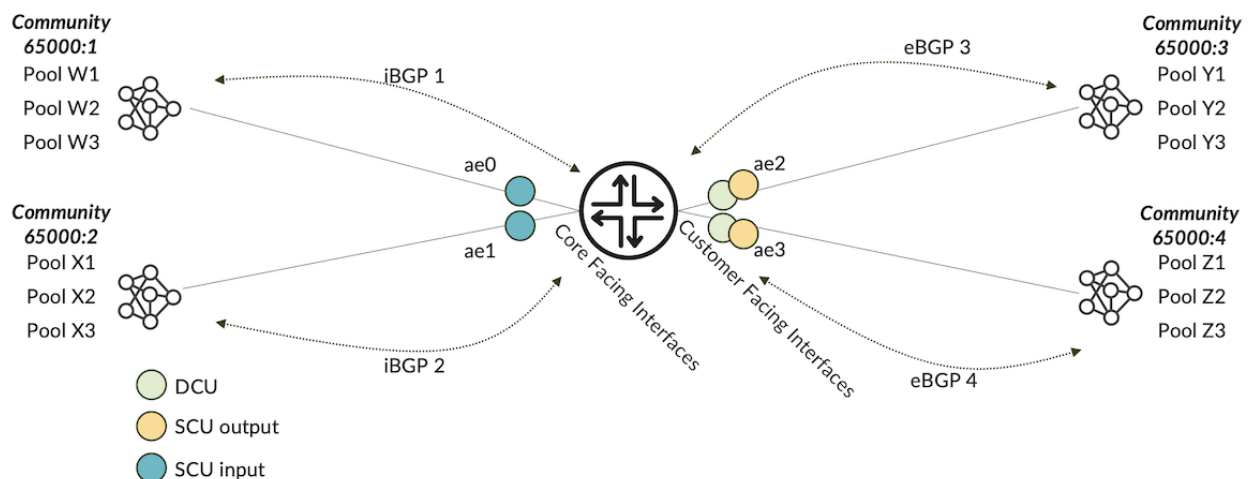
Figure 1: Simple SCU/DCU Illustration
