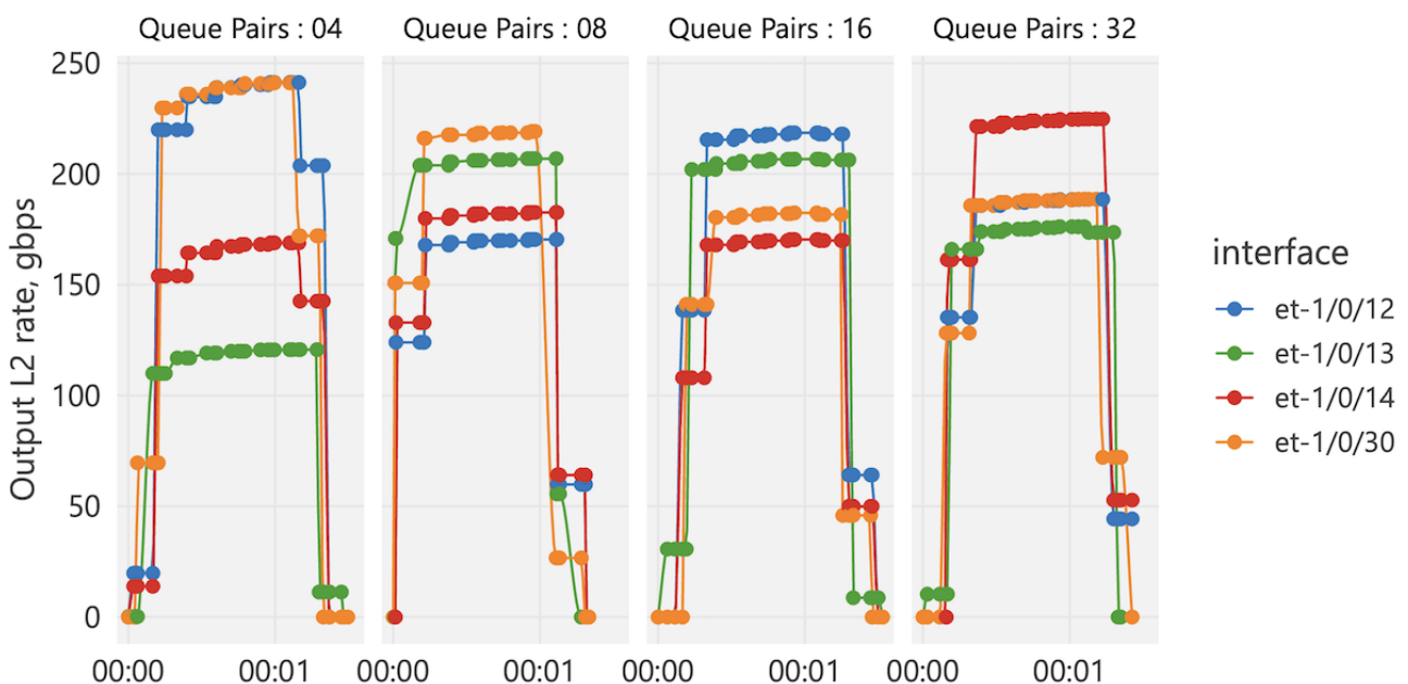
Figure 2: Interface rates with changing number of queue pairs NCCL setting.
