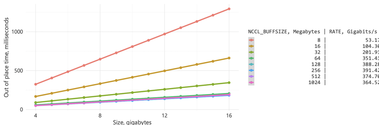
Figure 4: All reduce performance.
