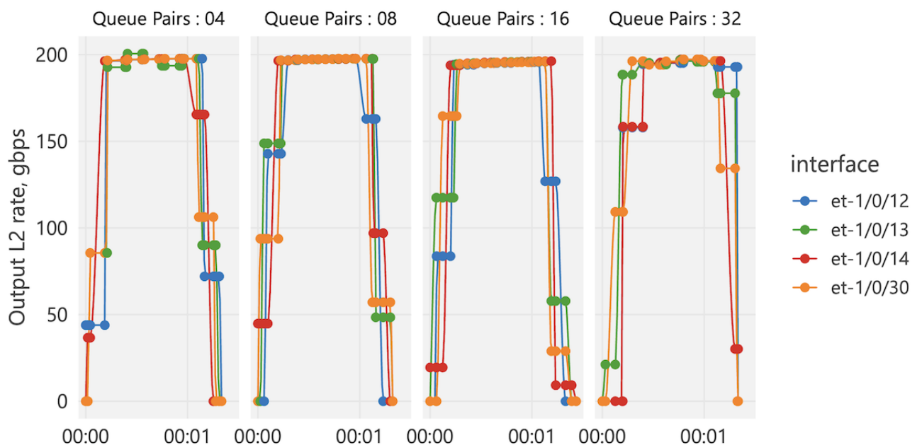
Figure 3: Figure 3. Interface rates with changing number of queue pairs NCCL setting. Adaptive Routing Enabled.
