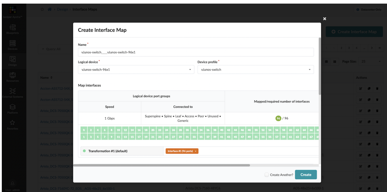
Figure 4: vJunos-switch Interface Map created in Apstra
