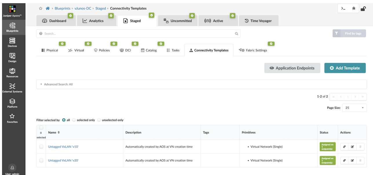
Figure 13: Connectivity Templates created in Apstra as part of VN creation
