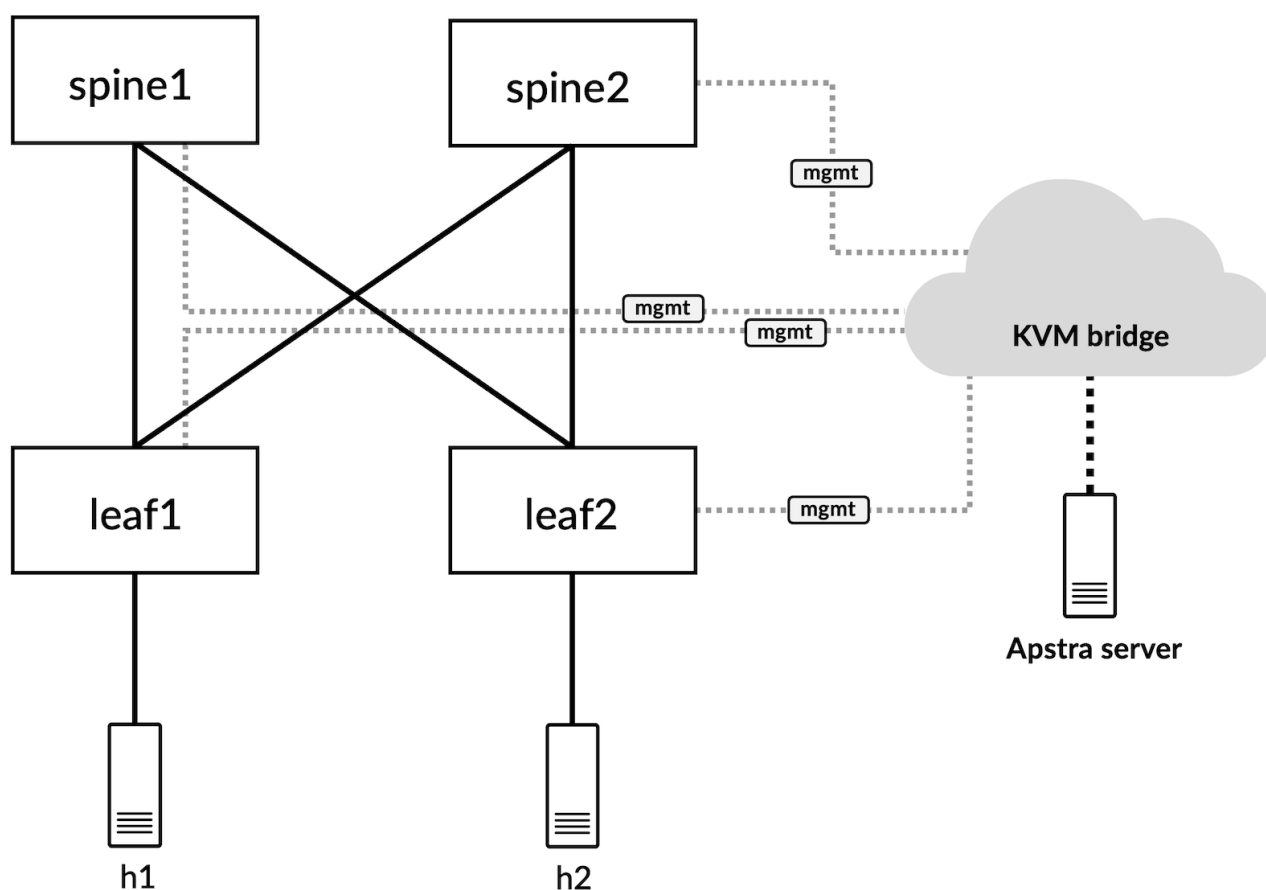
Figure 1: Network topology deployed via Containerlab
