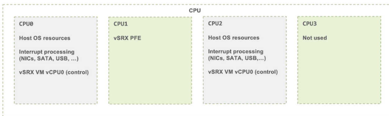
Figure 4: Sample split of CPU resources between tasks
