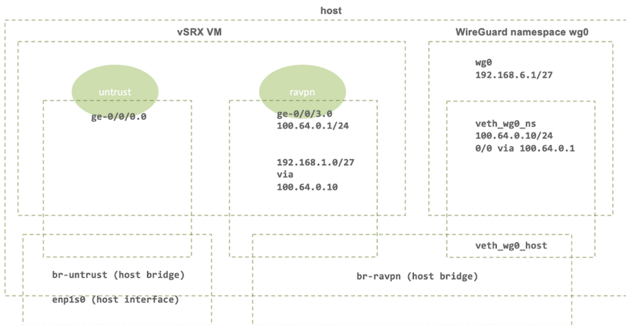
Figure 6: Sample layout of vSRX WireGuard network topology
