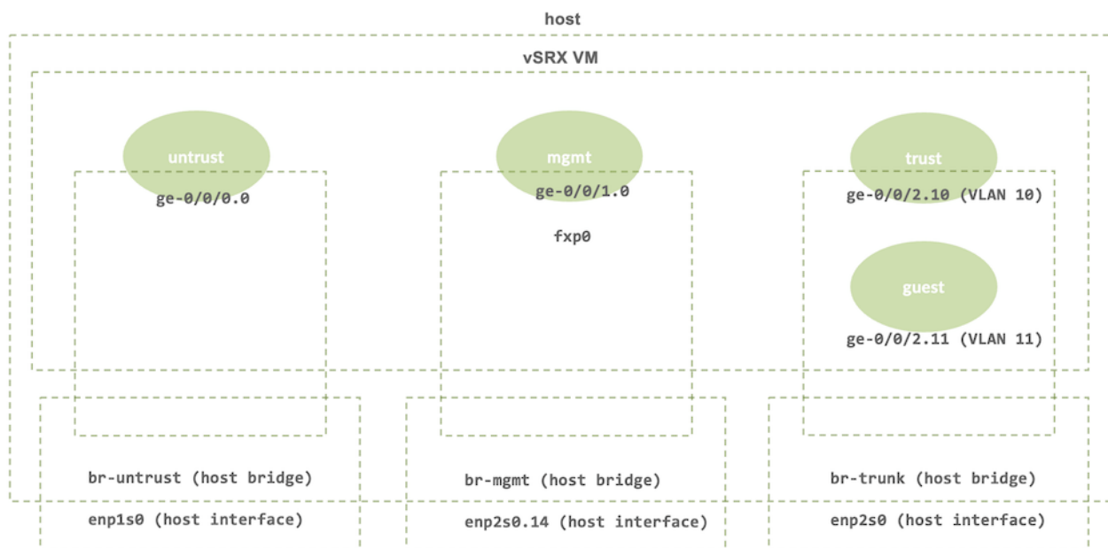
Figure 3: Sample layout of host OS and vSRX networking bindings
