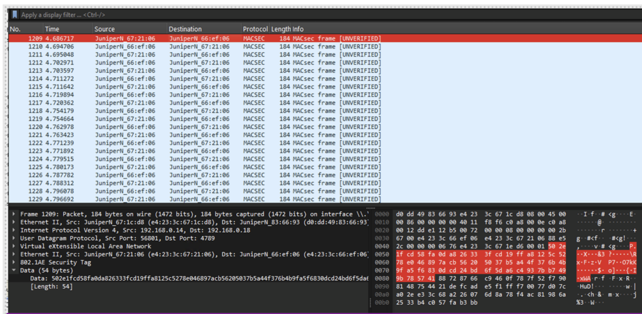
Figure 5: Packet Capture with VXLAN-Sec Enabled
