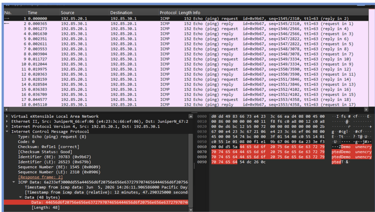
Figure 4: Packet Capture without VXLAN-Sec Enabled
