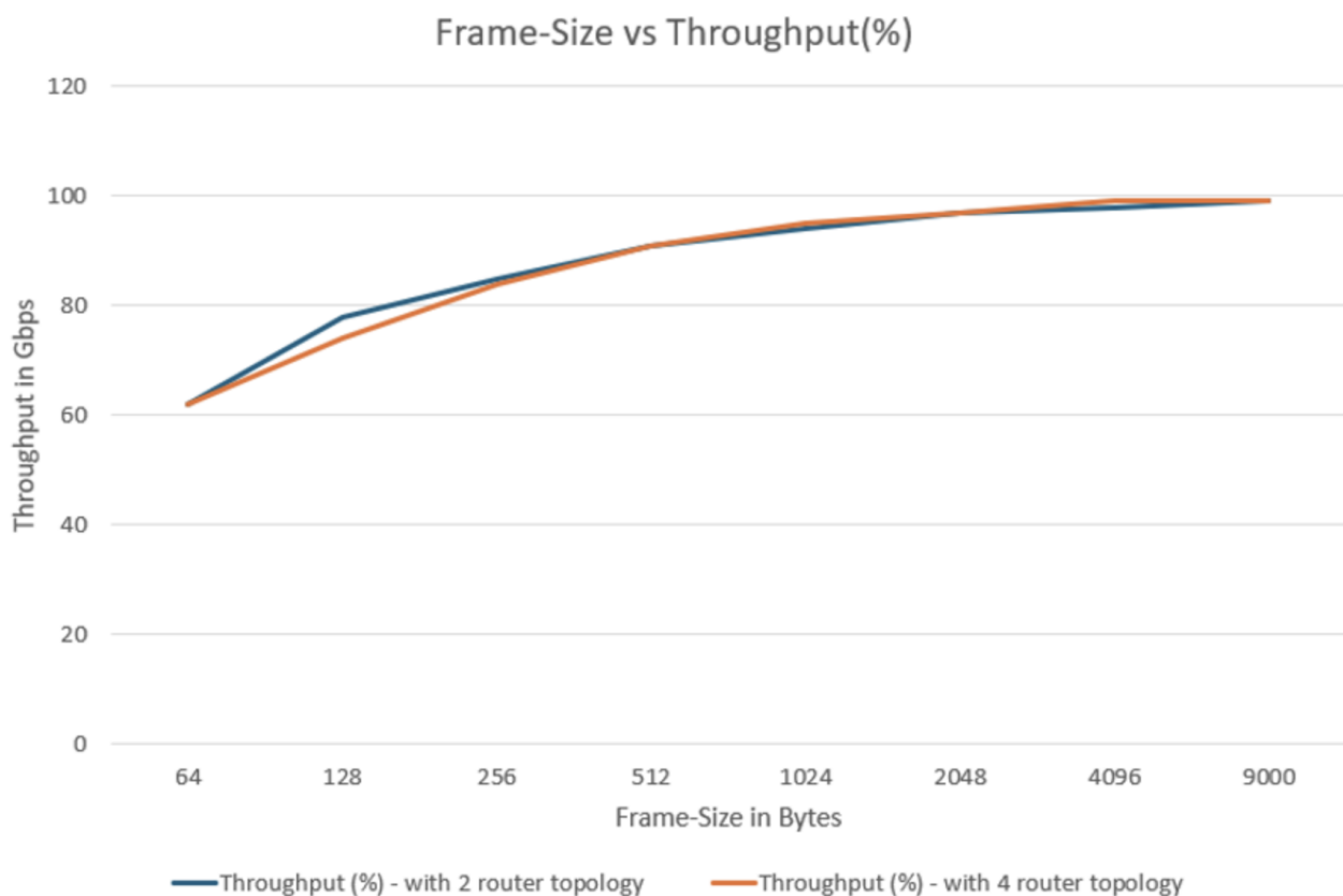
Figure 7: Throughput vs Frame Size for L3-stream
