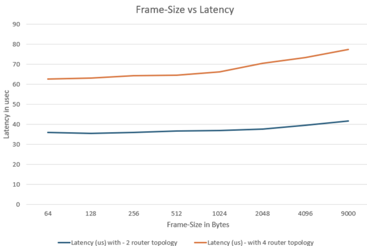
Figure 10: Average Latency vs Frame Size for L2-stream
