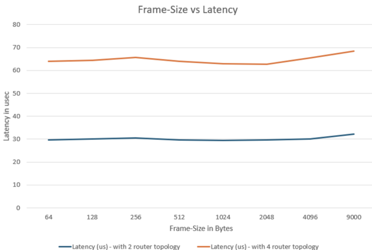
Figure 8: Average Latency vs Frame Size for L3-stream
