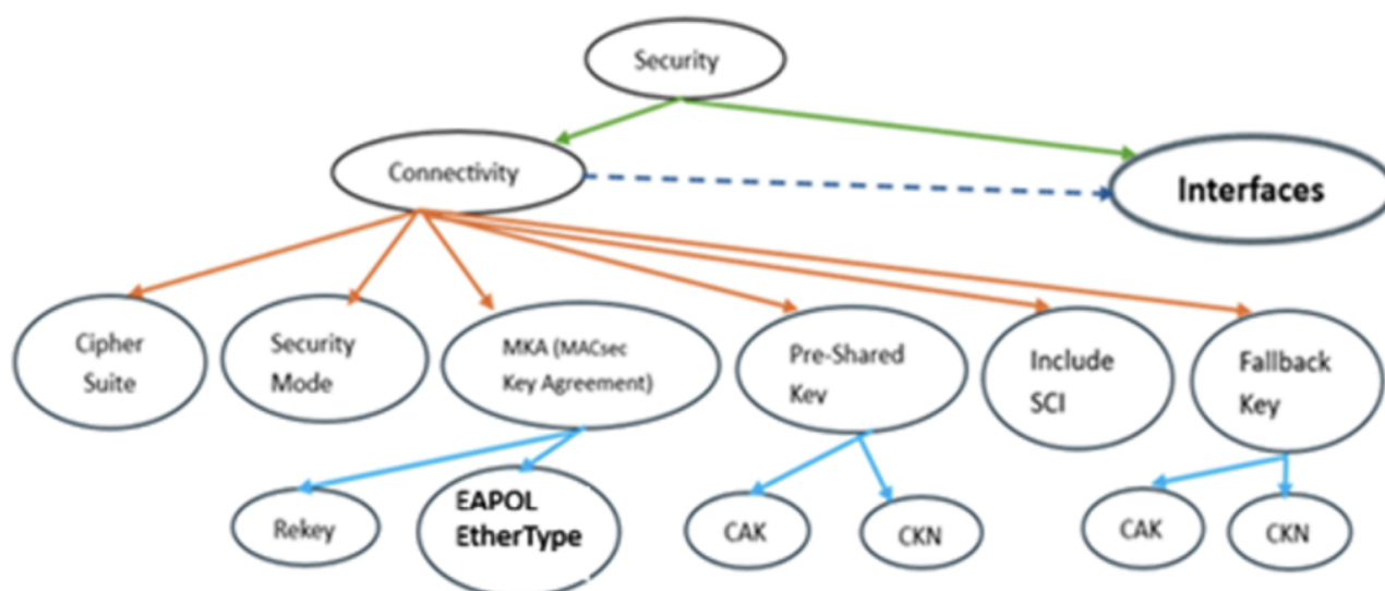
Figure 2: Bringing Up WAN-MACSec on MX Router
