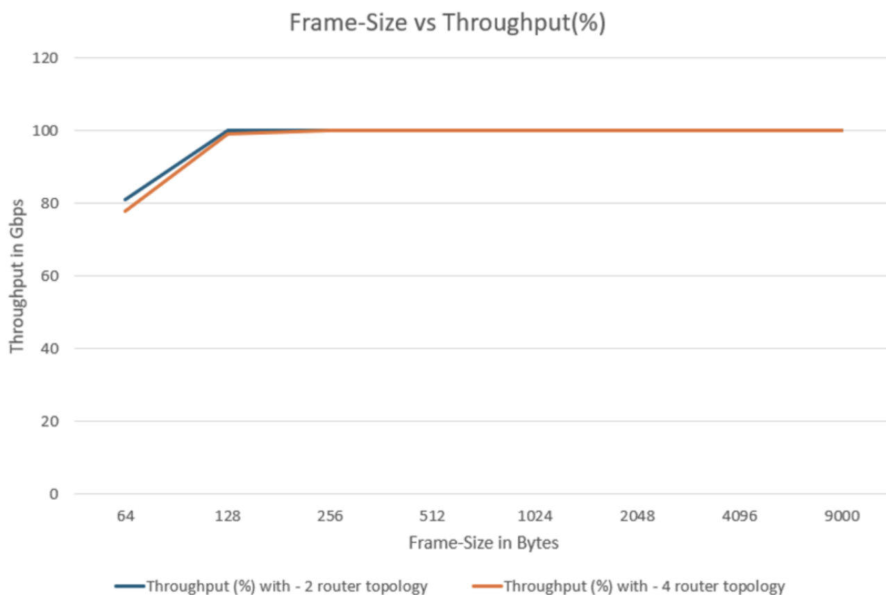
Figure 9: Throughput vs Frame Size for L2-stream
