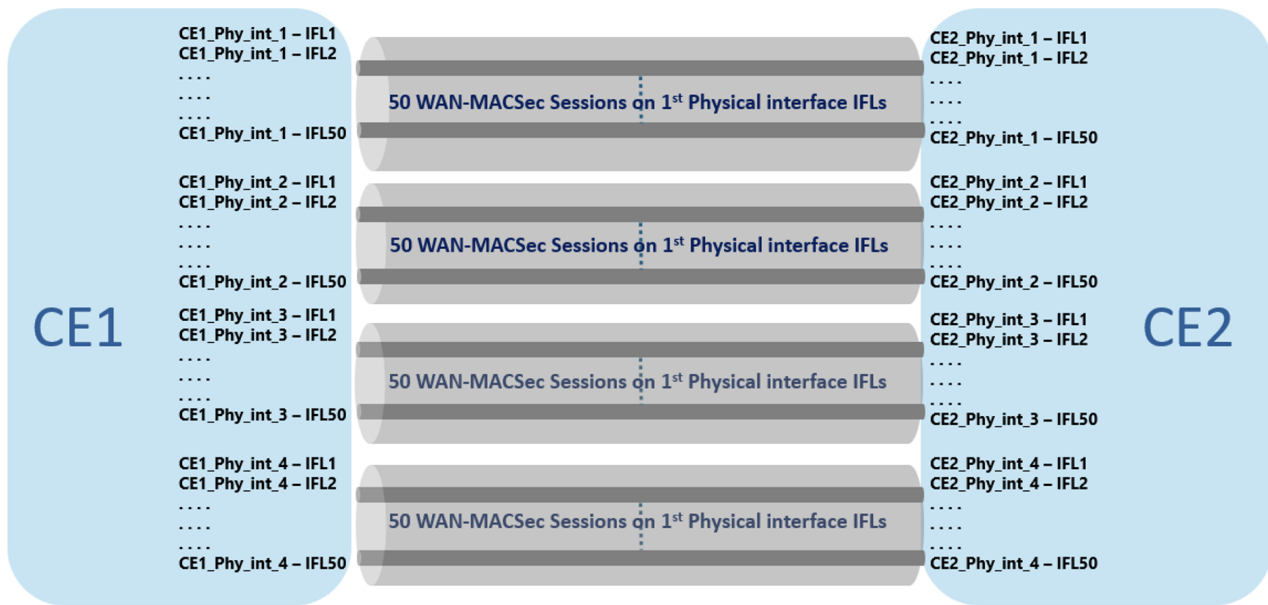
Figure 6: Scaled Logical topology
