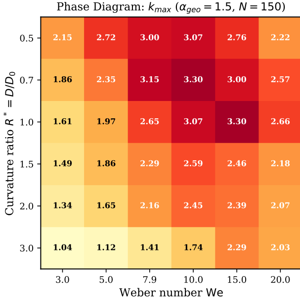
FIG. 3. Phase diagram: k_{max} as a function of We and R^* ( \alpha_{geo} = 1.5 , N = 150 , \theta_{eq} = 162^\circ ). Within the 2000-step window, asymmetry peaks near We \approx 15 at R^* \approx 1.0 . All cells are computed (see Table IV and the Supplementary Material).
