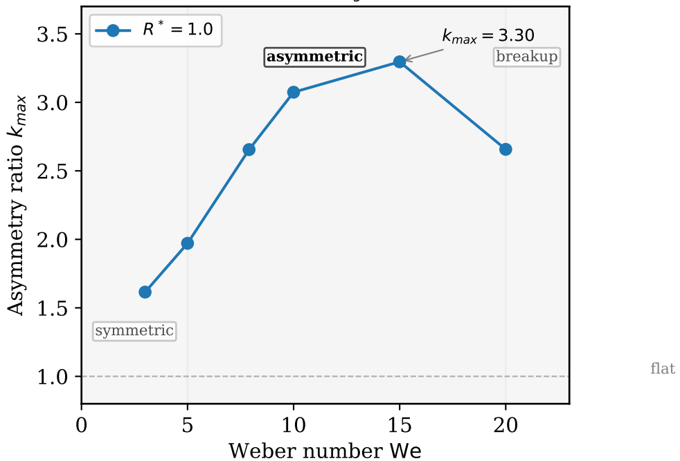
(a) k vs We ( R^* = 1.0 , \alpha_{geo} = 1.5 , N = 150 )
