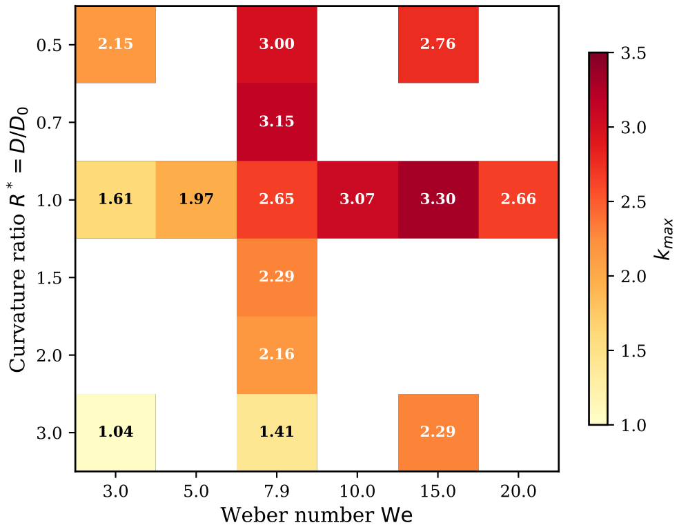
Phase Diagram: k_{\max} ( \alpha_{\text{geo}} = 1.5 , N = 150 )
