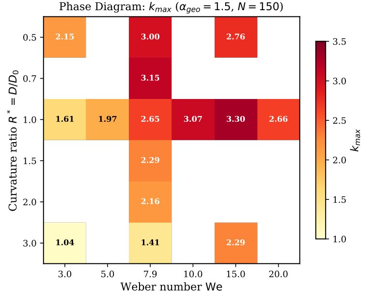
FIG. 3. Phase diagram: k_{max} as a function of We and R^* ( \alpha_{geo} = 1.5 , N = 150 ). Within the 2000-step window, asymmetry peaks near We \approx 15 at R^* \approx 1.0 . Empty cells indicate uncomputed parameter combinations.
