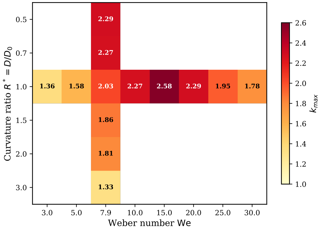
Phase Diagram: k_{max} ( \alpha_{geo} = 1.5 , N = 80 )
