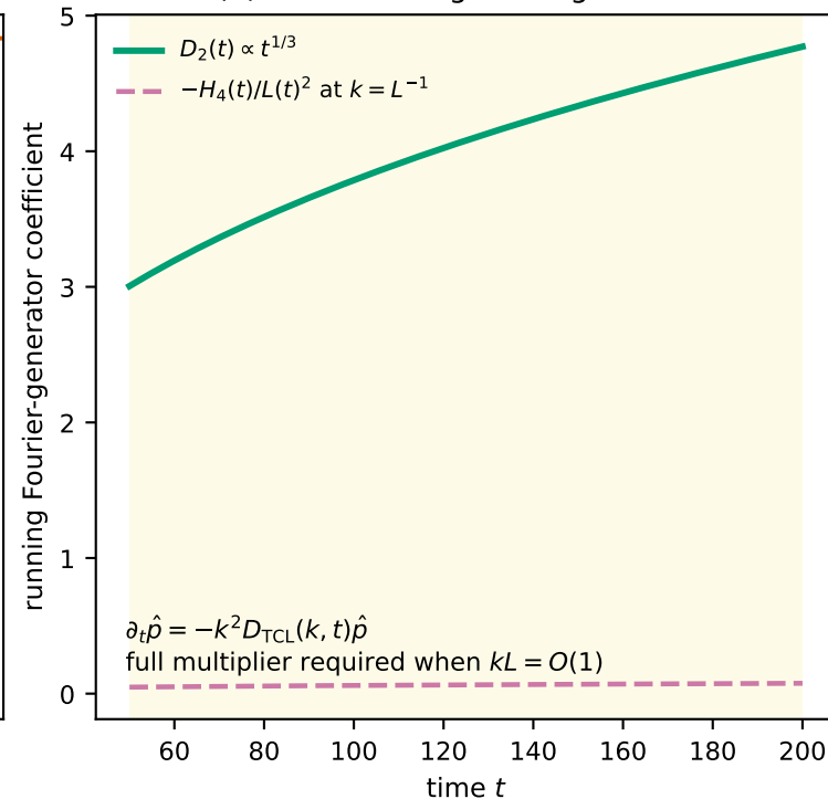
(b) Exact leading mean generator
