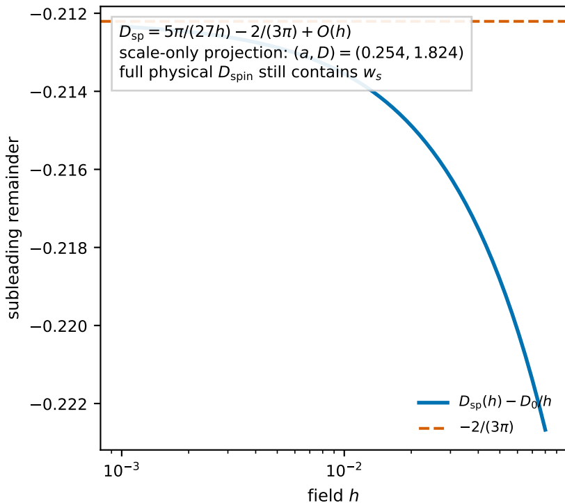
(a) Analytic finite-field regulator
