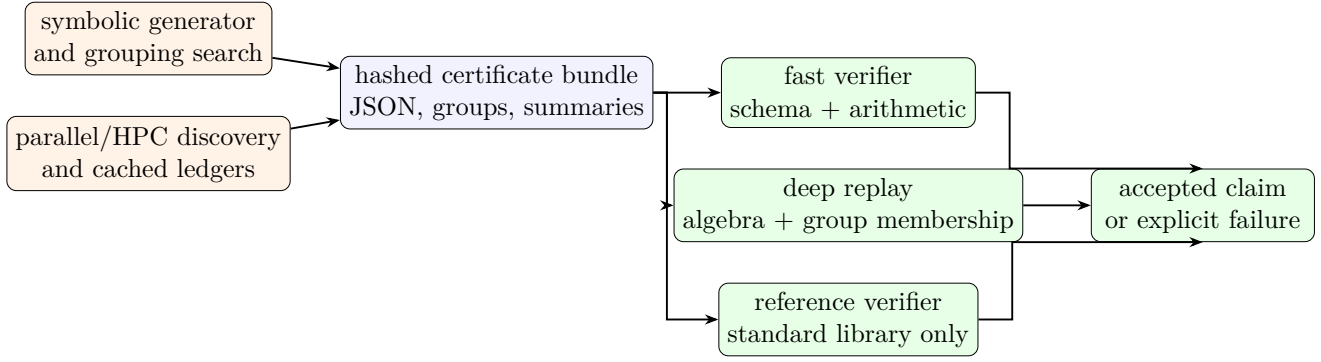
Figure 3: Trust boundary. Parallel discovery and heuristic grouping are untrusted producers. The accepted result depends on explicit evidence and three verification paths with different trust surfaces.
