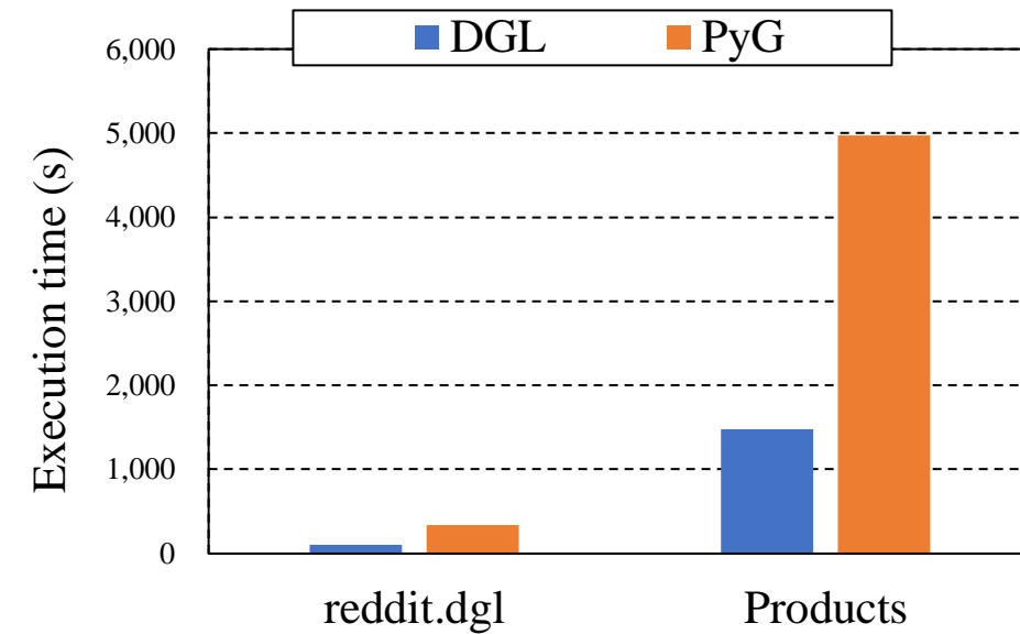
GraphSAGE
