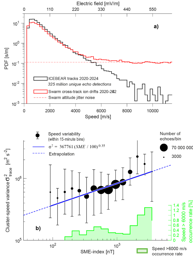
Figure 9. Panel a) shows, in a solid black line, the distribution of 74,517 clusters tracked by ICEBEAR during geomagnetically disturbed conditions (SME-index > 150 nT). The distribution of ion drifts speed derived from Swarm A EFI horizontal moments, during the same conditions and inside the auroral region ( 18h < MLT < 6h , 61^\circ < MLAT < 69^\circ ), is shown with a solid red line. A dashed red line indicates the noise limitation caused by spacecraft attitude jitter and anomalous spacecraft potential and calibration drift (Knudsen et al., 2017). Panel b) shows the same dataset, this time binning all the tracked clusters into 4190 bins of 15-minute length (for a total of 1045 hours of radar-time), then binning (for the second time) the standard deviations, \sigma , of the cluster speeds inside each window, for the 24 geomagnetic activity bins. Black circles with errorbars denote average \sigma in each geomagnetic activity bin, and a black dashed line shows the result of a linear regression (slope = 572 m/s/, Pearson correlation = 0.84). In green, on the right y-axis, the occurrence rate for speeds > 6000 m/s is shown for each geomagnetic activity bin.
