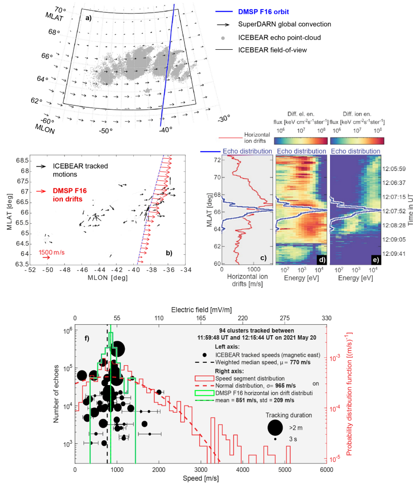
Figure 3. Conjunction between DMSP F16 and icebear on 20 May 2021. Panel a) shows DMSP F16 orbit (blue), superposed on a vector-field of SuperDARN global convection (black arrows) and ICEBEAR echo locations (gray dots). Panel b) shows the ICEBEAR tracked motions (black arrows) and the DMSP F16 horizontal ion drifts (red arrows). Panel c) shows the DMSP F16 horizontal ion drifts (red line), while panels d) and e) show the precipitating electron and ion differential energy flux, respectively, represented with a colorscale. In panels c–e), the latitudinal distribution of ICEBEAR echoes is superposed with a blue line. Panel f) shows, on the left y -axis, the distribution of tracked ICEBEAR clusters (black circles), taking the eastward component only, with a dashed black line giving the weighted median speed (770 m/s). On the right y -axis, the distributions in ICEBEAR per-frame displacements is shown in a solid red line, with a Gaussian fit displayed with a dashed red line ( \sigma = 965 m/s). The distribution in DMSP F16 ion drifts is shown with a green line, with a mean of 851 m/s and a standard deviation of 209 m/s.
