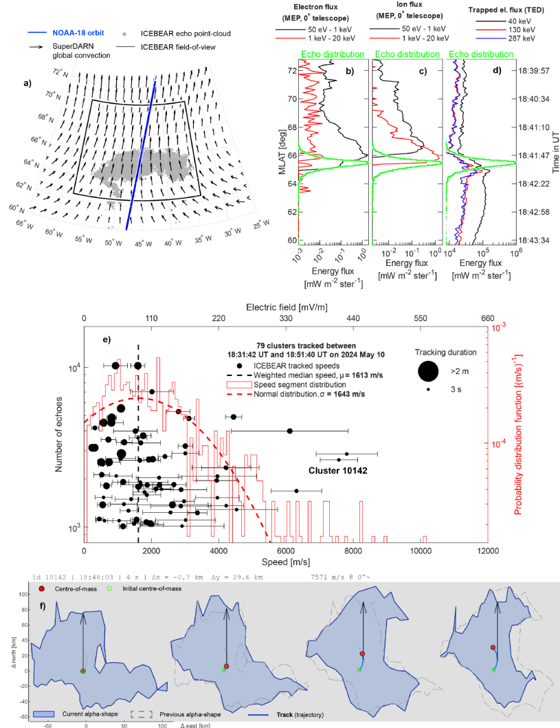
Figure 8. Conjunction between NOAA-18 and icebear at 18:30 UT on 10 May 2024. Panel a) shows NOAA-18's orbit (blue), superposed on a vector-field of SuperDARN global convection (black arrows) and ICEBEAR echo locations (gray dots). Panels b) and c) show the electron and ion fluxes measured by NOAA-18 (medium-energy, 0° telescopes), while panel d) shows the trapped particle fluxes. In panels b-d), the latitudinal distribution of ICEBEAR echoes is superposed with a green line. Panel e) shows the distribution of tracked ICEBEAR clusters (black circles) around the time of the conjunction. On the right y -axis, the distributions in ICEBEAR velocity segments is shown in a solid red line, with a Gaussian fit displayed with a dashed red line ( \sigma = 1643 m/s). Cluster 10142 is indicated, whose evolution is shown in detail in panel f) , akin to Figure 6.
