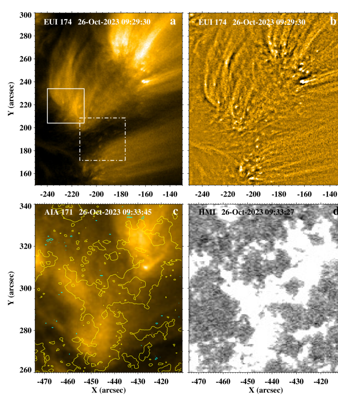
Figure 9. An example of network microflashes at a plume-base observed by HRIEUV and SDO on 26-October-2023. Panel (a) shows HRIEUV 174 Å image of solar plumes and microflashes. Panel (b) shows the unsharp mask version of the same image. Panel (c) shows the same FOV in AIA 171 Å. Panel (d) shows the line-of-sight photospheric magnetic flux in the same FOV. In panel (c), HMI contours, of levels \pm 20 G, at 09:33:27 UT are overlaid, where yellow and cyan contours outline positive and negative magnetic flux, respectively. The solid white box and dotted-dashed white box in (a) outlines the FOV in Figures 10 and 11, respectively. The animation (Movie1) runs from 09:00 to 11:00 UT. The animation is unannotated and the FOV is same as in Panel (a).
