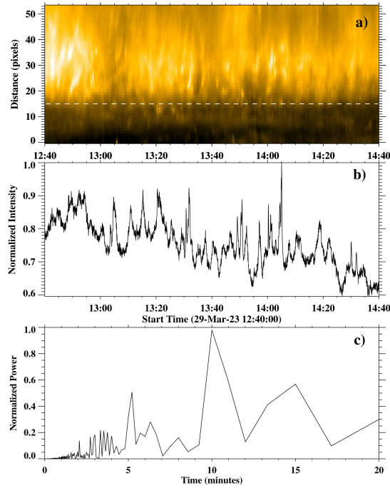
Figure 2. Examination of the periodicity of network microflashes. Panel (a) shows the HRIEUV 174 Å total intensity time-distance map plotted along the rectangular slit of Figure 1a. The right-leaning bright structures are the microflashes and their upflows that appear within that slit. Panel (b) shows the HRIEUV 174 Å intensity time profile from the white-dashed line in panel (a). The time profile shows peaks at intervals of 5–15 minutes. Panel (c) shows the power spectrum of the intensity time profile in (b).
