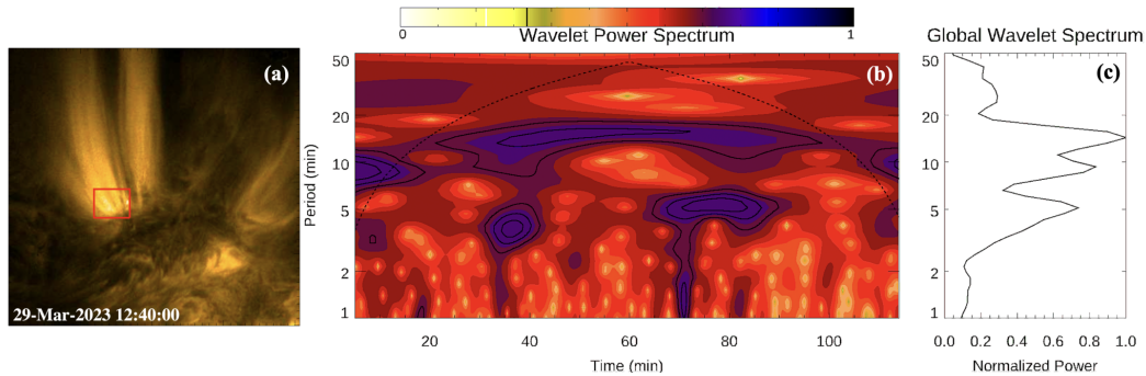
Figure 8. Results from the wavelet analysis. Panel (a) shows an \text{HRI}_{\text{EUV}} 174 Å image and the red box shows the region that was analyzed. Panel (b) shows the normalized wavelet power spectrum, inside the red box of (a), as function of time and period. The wavelet spectrum shows the power as a function of time and period, over the time of the \text{HRI}_{\text{EUV}} observations. The black dashed curve depicts the cone of influence the values outside of which are subject to edge effects and are considered unreliable. Panel (c) plots the normalized power-spectrum given by time integral of panel (b).
