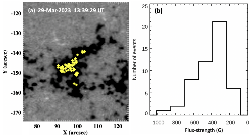
Figure 4. Magnetic Setting and Flux-strength histogram of 50 random manually selected microflashes. (a) Locations of the peak-brightness centroids of the 50 microflashes, marked by yellow "+" symbols, overlaid on the HMI plume-base flux map. (b) Histogram of HMI flux-strengths measured at the 50 microflash centroids shown in panel (a).
