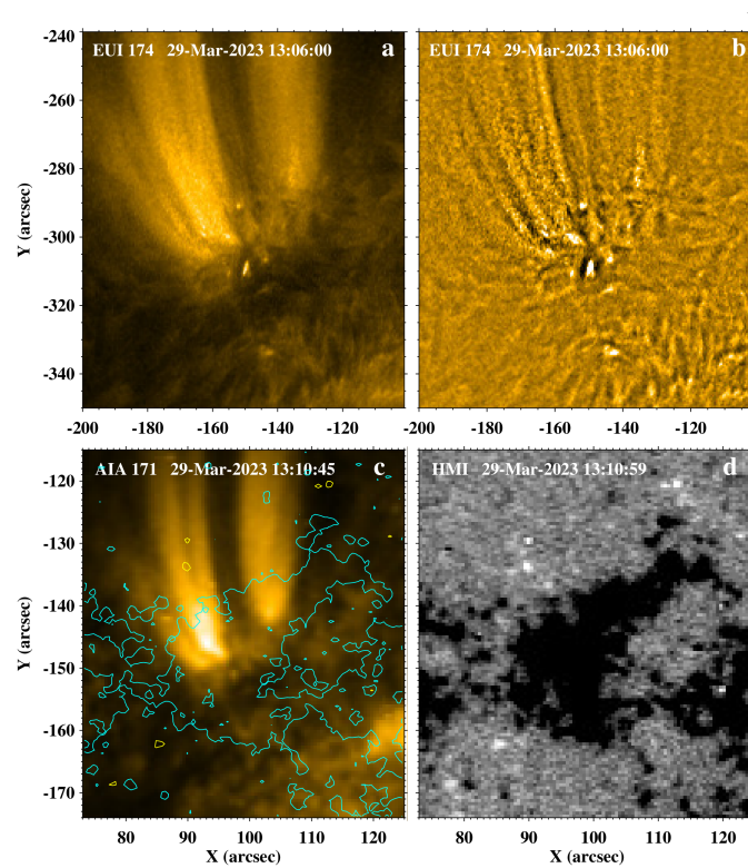
Figure 6. The first example of network microflashes at a plume base observed by HRIEUV (from Figure 1) and SDO. Panel (a) shows an HRIEUV 174 Å image of solar plumes and microflashes. Panel (b) shows the unsharp mask version of the same image. Panel (c) shows the same FOV in AIA 171 Å. Panel (d) shows the line-of-sight photospheric magnetic flux in the same FOV. In panel (c), HMI contours, of levels \pm 20 G, at 09:33:27 UT are overlaid, where yellow and cyan contours outline positive and negative magnetic flux, respectively. The animation (Movie2) runs from 12:40 to 14:40 UT. The animation is unannotated and the FOV is same as in Panel (a).
