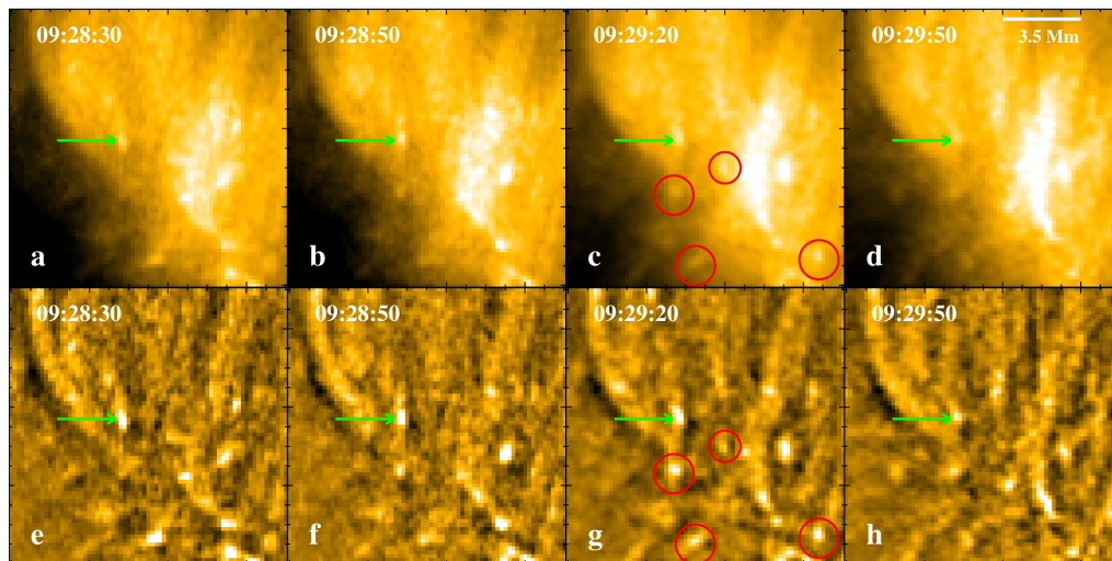
Figure 10. Network microflashes at the base of a plume. Panels (a–d) show 174 Å HRIEUV images of the plume base region in the FOV that is shown within the solid white box region of Figure 9a. Panels (e–h) show the unsharp mask images of the same. The green arrows point to a network microflash through most of its life. The red circles enclose other microflashes that are visible in these HRIEUV frames.
