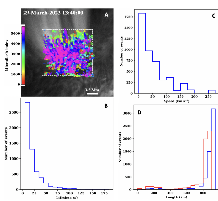
Figure 3. Automated detection of network microflashes. The different colored circles in panel (a) mark different microflashes detected over the entire HRI EUV time span. The white dashed region is the FOV searched for microflashes. The background image is the HRI EUV image at 13:40:00. Each microflash is indexed (1~6000) by its time of appearance, with color indicating detection time from red (earliest) to pink (latest), in accord with the corresponding color bar in (a). Panels (b–d) show histograms of microflash speed, lifetime, length (blue) and width (red), respectively, from the automated detection method. The mean values of the speed, lifetime, length and width are 50 \pm 50 \text{ km s}^{-1} , 22 \pm 20 \text{ seconds} , 860 \pm 150 \text{ km} and 770 \pm 200 \text{ km} , respectively.
