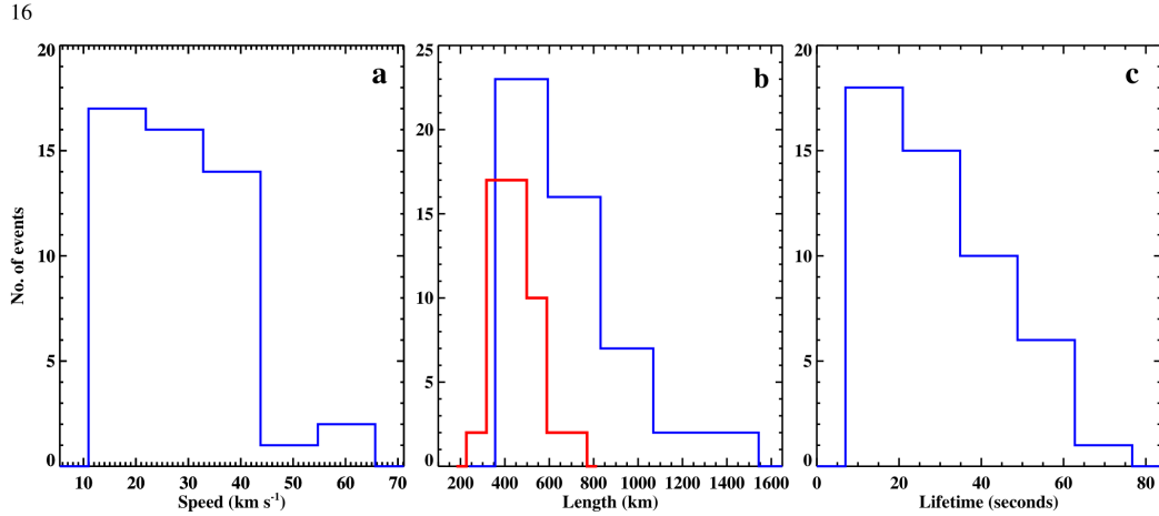
Figure 7. Histograms of the plane-of-sky speed (a), length (b), and lifetime (c) for the 50 manually selected network microflashes. The red histogram in (b) is the width of the microflashes. The bin size is different for length (235 km) and width (100 km) histograms. The mean values of the speed, length, width, and lifetime are 27.5 \pm 11.5 km s -1 , 675 \pm 250 km, 450 \pm 95 km, and 30 \pm 15 seconds, respectively.
