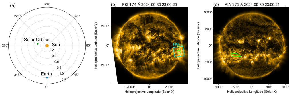
Fig. 1. Overview of the positions (a) and viewing geometry from Solar Orbiter (b), and SDO (c). The cyan square denotes the field of view (FoV) of HRI EUV . Since the HRI EUV FoV partially lies outside the solar disk, we define a smaller on-disk region (green square) within the FoV and re-project this region onto the SDO perspective.
