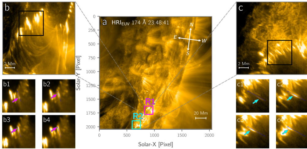
Fig. 2. Overview of the downflows in this event. Panel (a) shows the field of view of the HRI EUV observation. The boxes labeled R1 and R2 mark two different flare-ribbon regions. Panels (b) and (c) present zoomed-in views of regions R1 and R2. Panels (b1–b4) and (c1–c4) display the detailed temporal evolution of two selected individual downflows. The fields of view of these panels are indicated by the black squares in panels (b) and (c), respectively. The blue arrows indicate the trajectories of the downflows. The pink and cyan arrows mark the locations of the downflows in the corresponding frame.
