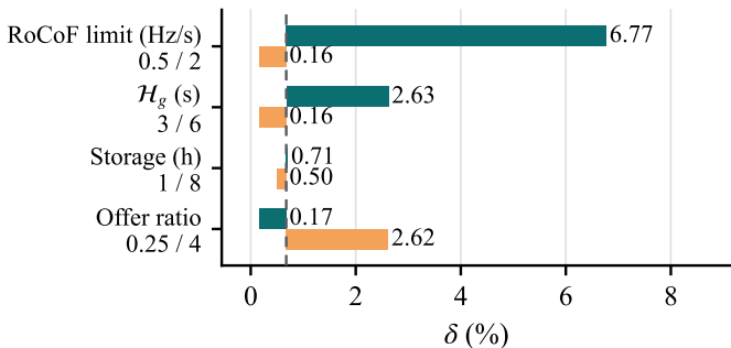
RTS-24, 20%: base \delta = 0.68\%
