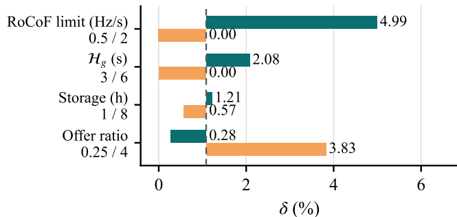
RTS-24, 40%: base \delta = 1.08\%
