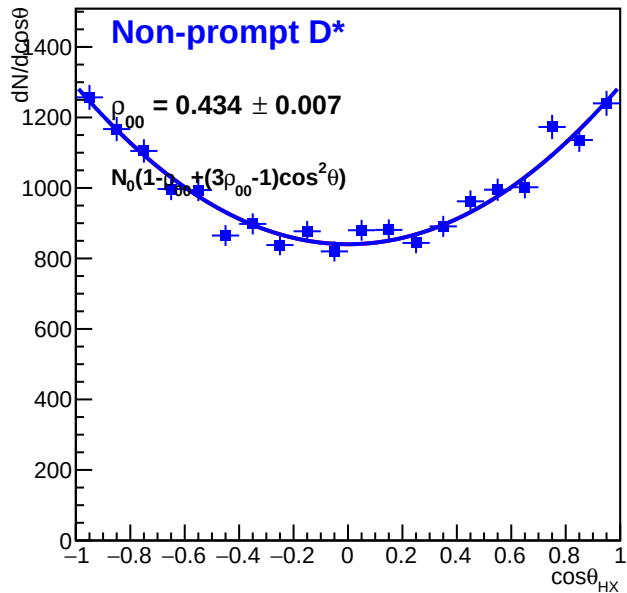
Non-prompt D* ( 10 < p_T < 20 GeV/c)
