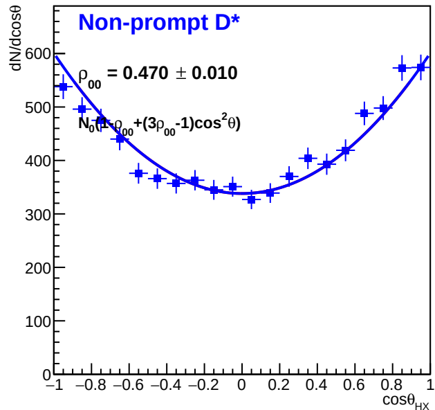
Non-prompt D* ( 20 < p_T < 50 GeV/c)
