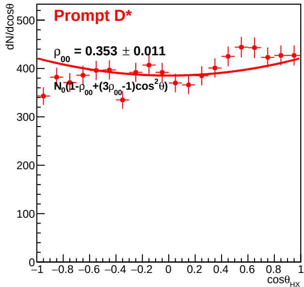
Prompt D* ( 20 < p_T < 50 GeV/c)
